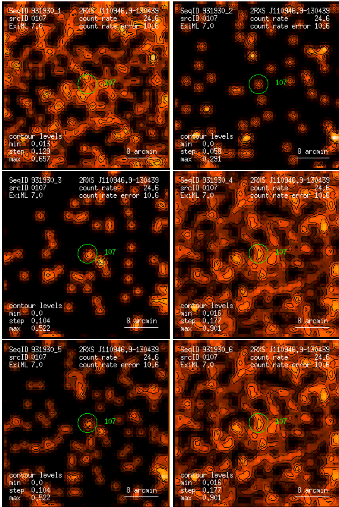
Figure 107: RASS 931930: detection 0107: band rate images, Gaussian filter: (1) PSPC channels 11 – 41, (2) 52 – 90, (3) 91 – 201, (4) 11 – 235, (5) 52 – 201, (6) 11 – 201. Broad band rates in counts/ks. Band rate contour levels in counts/ks/arcmin 2 .
