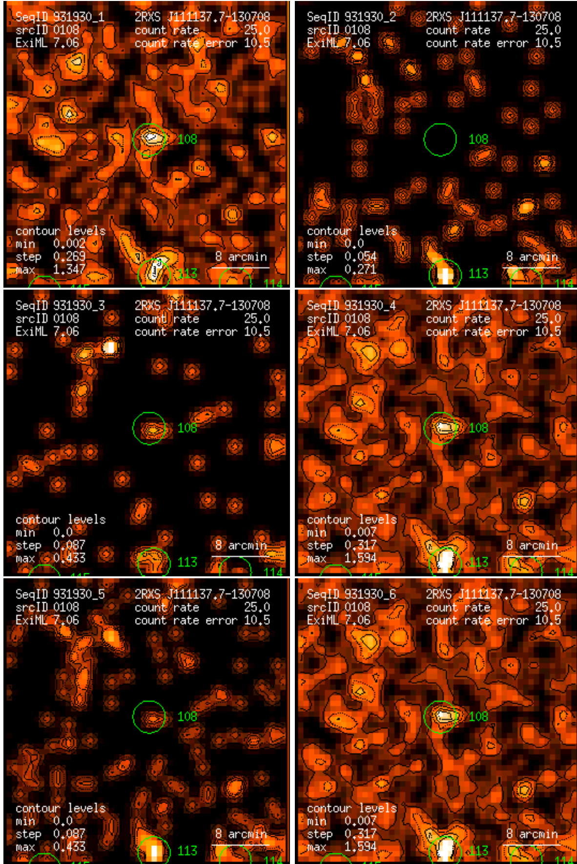
Figure 108: RASS 931930: detection 0108: band rate images, Gaussian filter: (1) PSPC channels 11 – 41, (2) 52 – 90, (3) 91 – 201, (4) 11 – 235, (5) 52 – 201, (6) 11 – 201. Broad band rates in counts/ks. Band rate contour levels in counts/ks/arcmin 2 .
