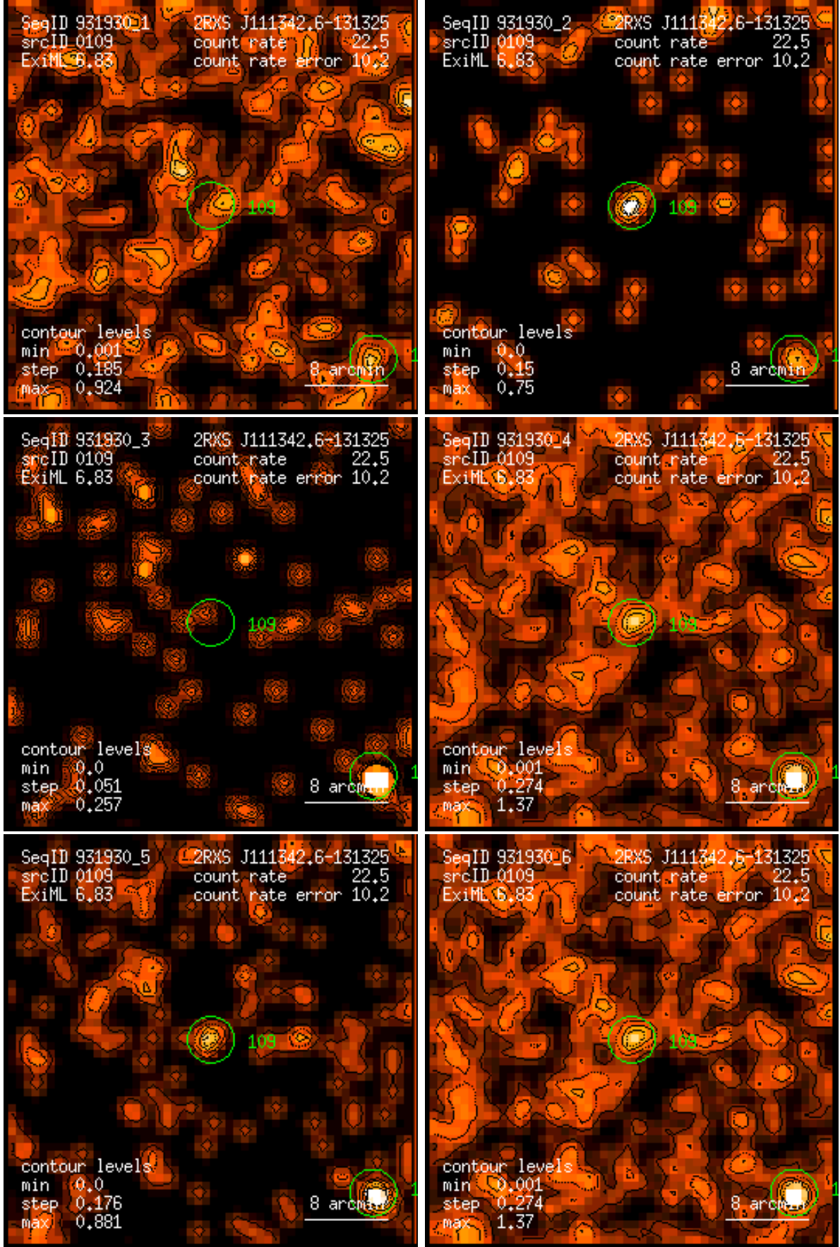
Figure 109: RASS 931930: detection 0109: band rate images, Gaussian filter: (1) PSPC channels 11 – 41, (2) 52 – 90, (3) 91 – 201, (4) 11 – 235, (5) 52 – 201, (6) 11 – 201. Broad band rates in counts/ks. Band rate contour levels in counts/ks/arcmin 2 .
