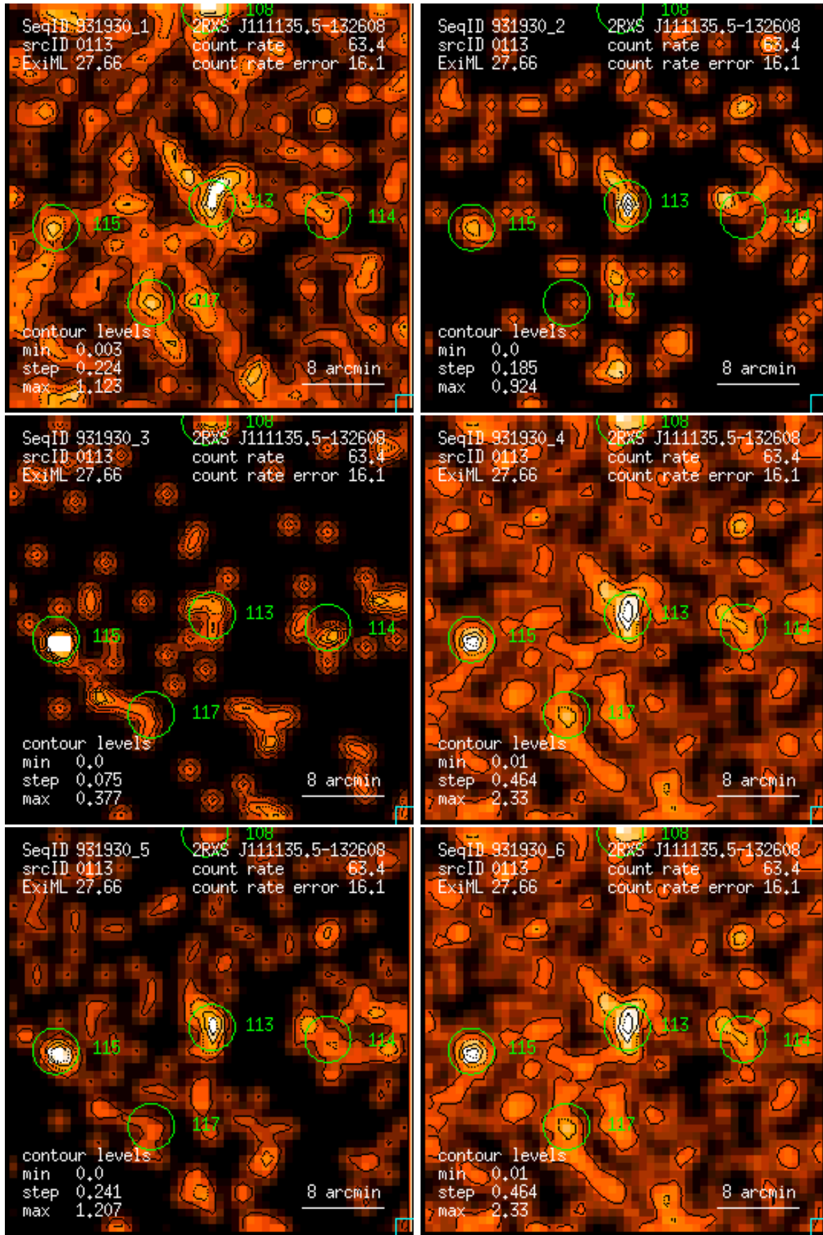
Figure 113: RASS 931930: detection 0113: band rate images, Gaussian filter: (1) PSPC channels 11 – 41, (2) 52 – 90, (3) 91 – 201, (4) 11 – 235, (5) 52 – 201, (6) 11 – 201. Broad band rates in counts/ks. Band rate contour levels in counts/ks/arcmin 2 .
