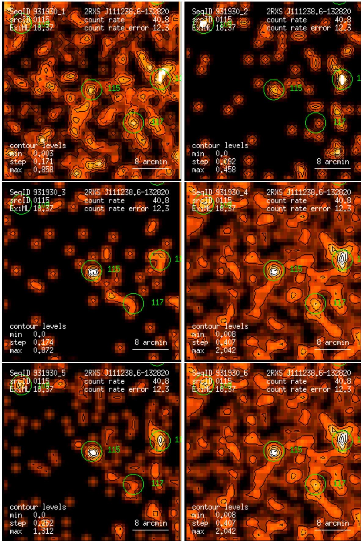
Figure 115: RASS 931930: detection 0115: band rate images, Gaussian filter: (1) PSPC channels 11 – 41, (2) 52 – 90, (3) 91 – 201, (4) 11 – 235, (5) 52 – 201, (6) 11 – 201. Broad band rates in counts/ks. Band rate contour levels in counts/ks/arcmin 2 .
