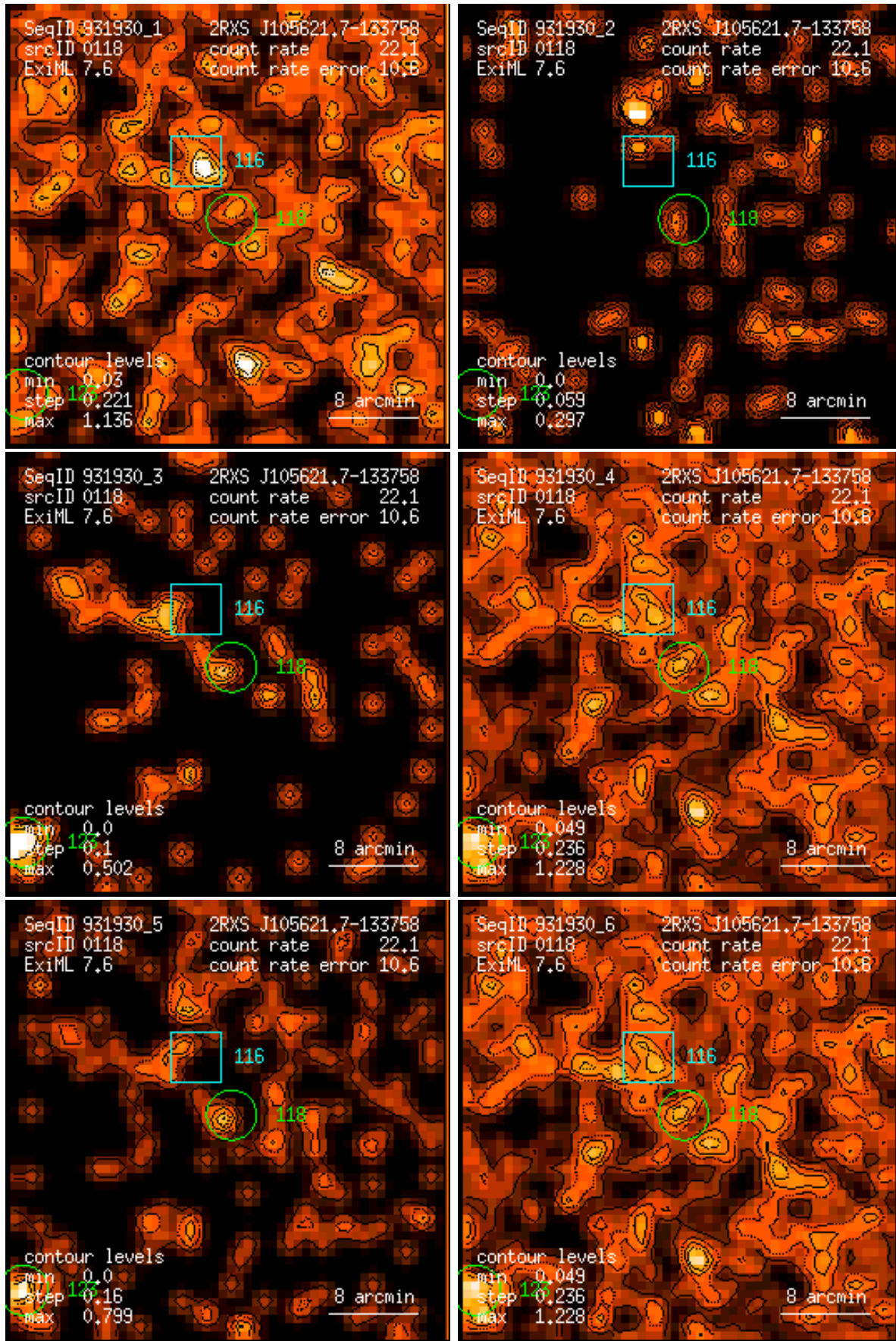
Figure 118: RASS 931930: detection 0118: band rate images, Gaussian filter: (1) PSPC channels 11 – 41, (2) 52 – 90, (3) 91 – 201, (4) 11 – 235, (5) 52 – 201, (6) 11 – 201. Broad band rates in counts/ks. Band rate contour levels in counts/ks/arcmin 2 .
