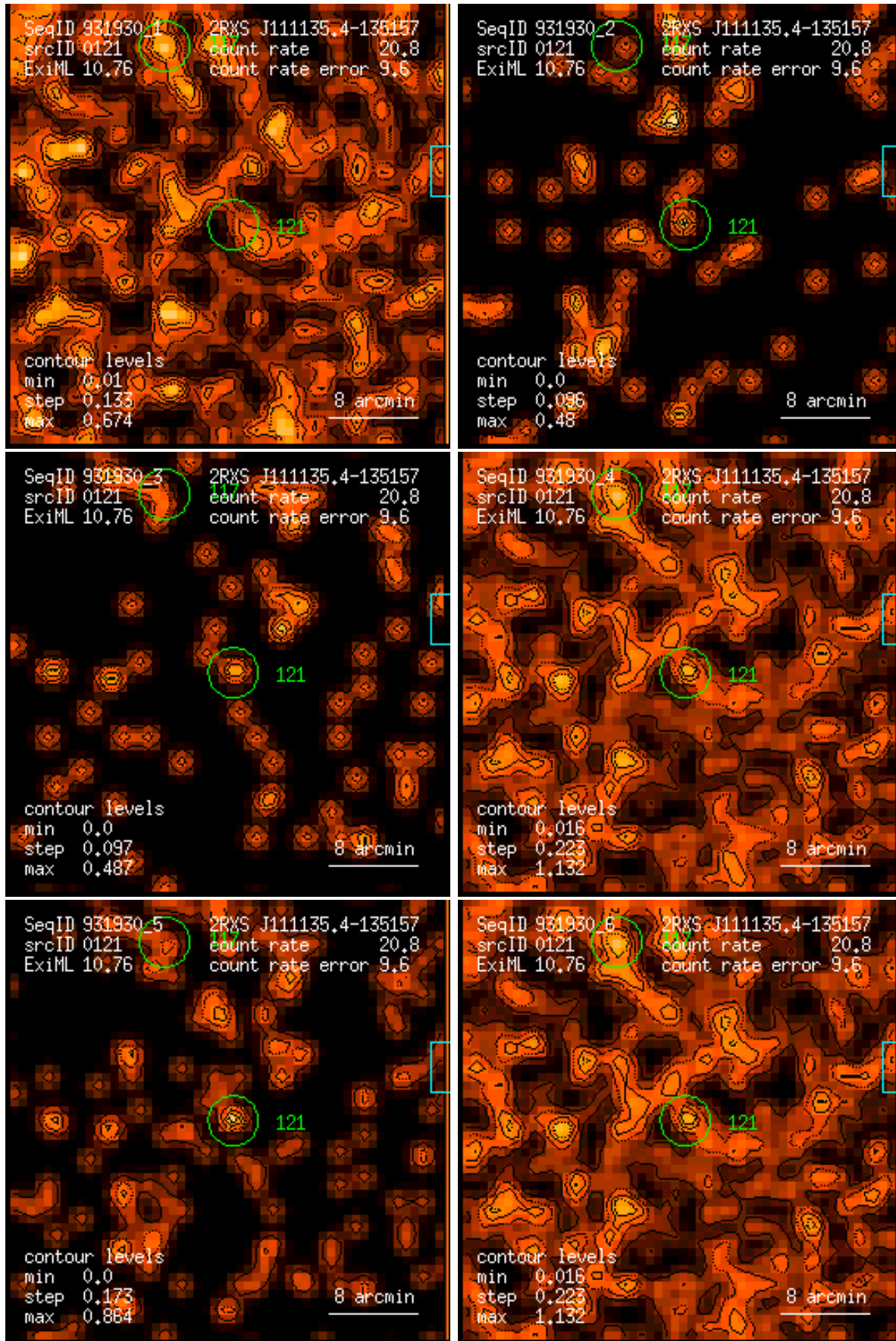
Figure 121: RASS 931930: detection 0121: band rate images, Gaussian filter: (1) PSPC channels 11 – 41, (2) 52 – 90, (3) 91 – 201, (4) 11 – 235, (5) 52 – 201, (6) 11 – 201. Broad band rates in counts/ks. Band rate contour levels in counts/ks/arcmin 2 .
