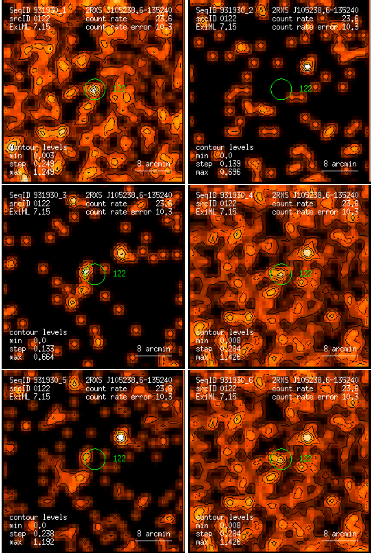
Figure 122: RASS 931930: detection 0122: band rate images, Gaussian filter: (1) PSPC channels 11 – 41, (2) 52 – 90, (3) 91 – 201, (4) 11 – 235, (5) 52 – 201, (6) 11 – 201. Broad band rates in counts/ks. Band rate contour levels in counts/ks/arcmin 2 .
