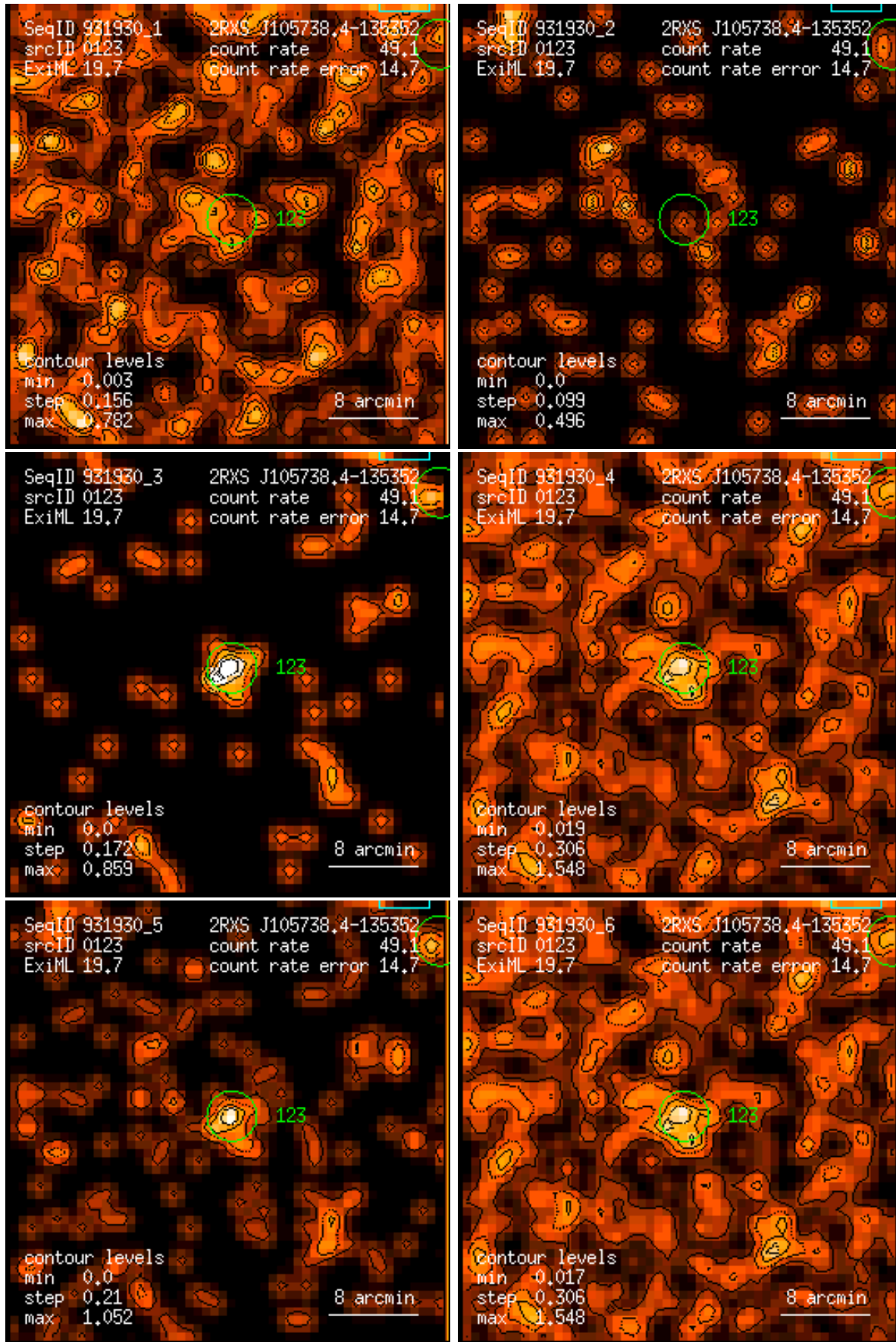
Figure 123: RASS 931930: detection 0123: band rate images, Gaussian filter: (1) PSPC channels 11 – 41, (2) 52 – 90, (3) 91 – 201, (4) 11 – 235, (5) 52 – 201, (6) 11 – 201. Broad band rates in counts/ks. Band rate contour levels in counts/ks/arcmin 2 .
