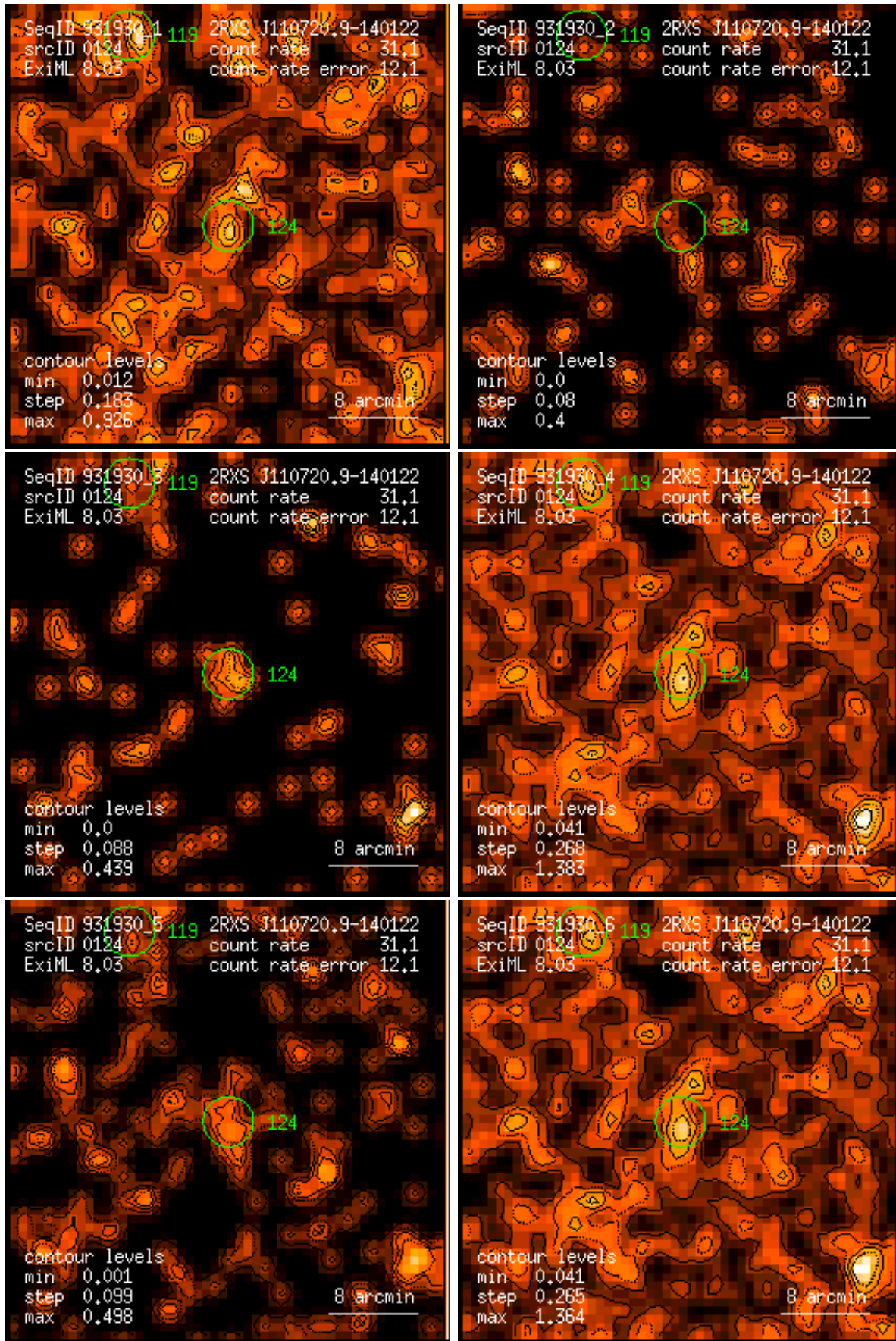
Figure 124: RASS 931930: detection 0124: band rate images, Gaussian filter: (1) PSPC channels 11 – 41, (2) 52 – 90, (3) 91 – 201, (4) 11 – 235, (5) 52 – 201, (6) 11 – 201. Broad band rates in counts/ks. Band rate contour levels in counts/ks/arcmin 2 .
