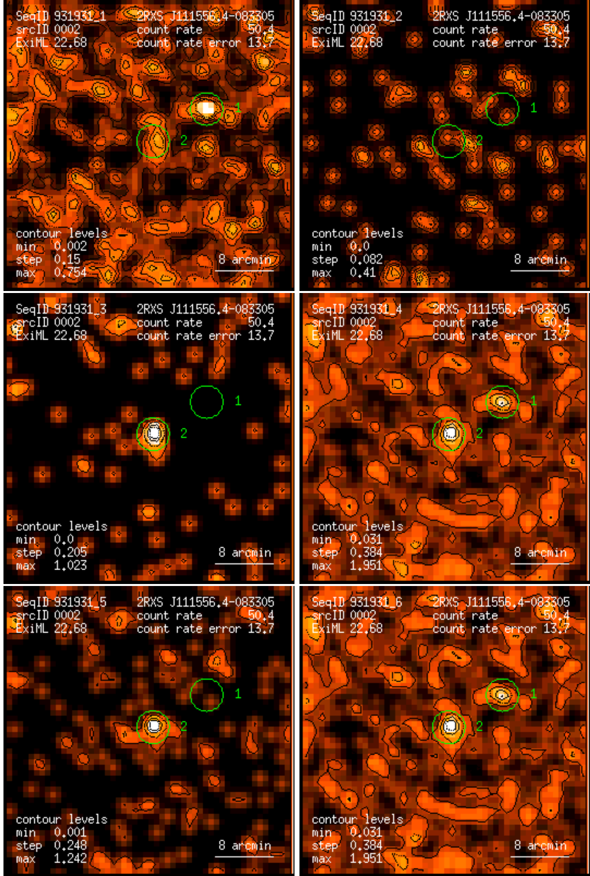
Figure 2: RASS 931931: detection 0002: band rate images, Gaussian filter: (1) PSPC channels 11 – 41, (2) 52 – 90, (3) 91 – 201, (4) 11 – 235, (5) 52 – 201, (6) 11 – 201. Broad band rates in counts/ks. Band rate contour levels in counts/ks/arcmin 2 .
