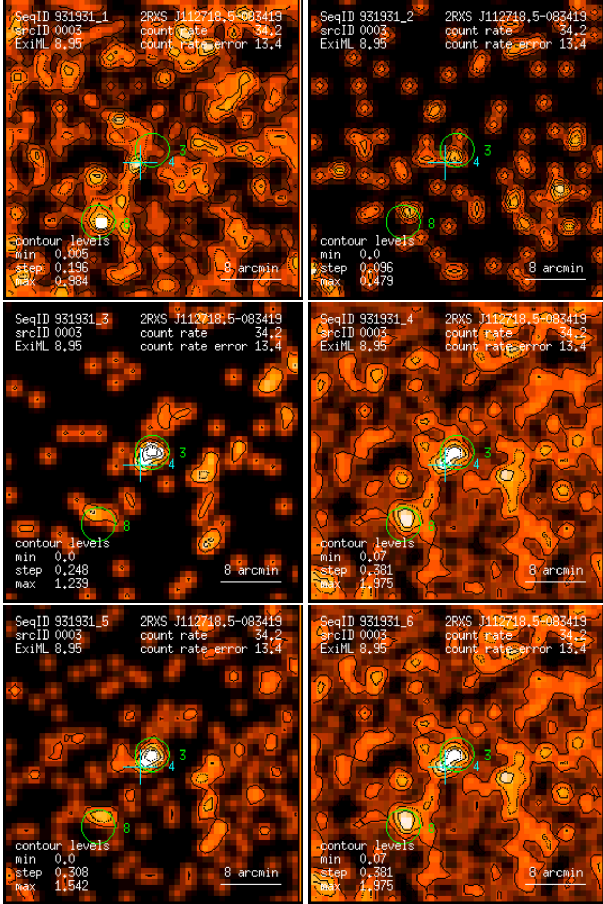
Figure 3: RASS 931931: detection 0003: band rate images, Gaussian filter: (1) PSPC channels 11 – 41, (2) 52 – 90, (3) 91 – 201, (4) 11 – 235, (5) 52 – 201, (6) 11 – 201. Broad band rates in counts/ks. Band rate contour levels in counts/ks/arcmin 2 .
