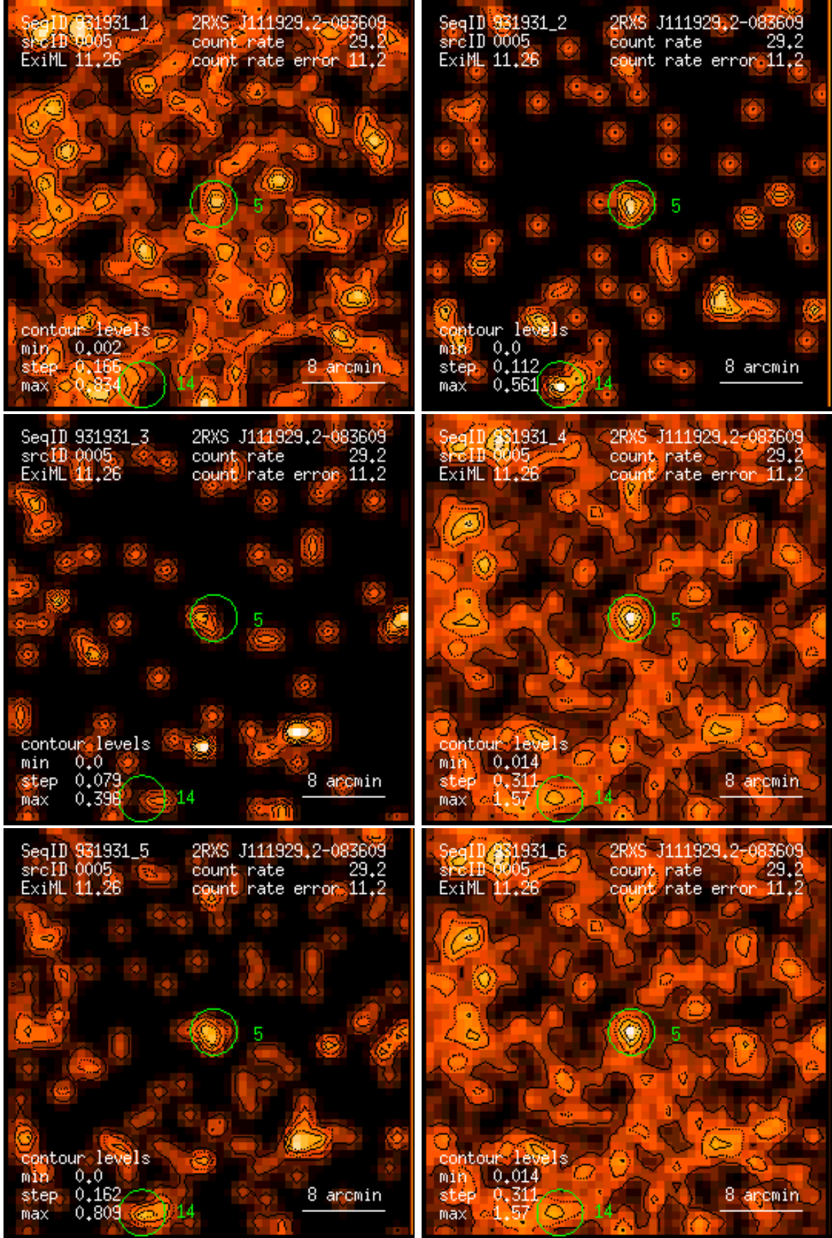
Figure 5: RASS 931931: detection 0005: band rate images, Gaussian filter: (1) PSPC channels 11 – 41, (2) 52 – 90, (3) 91 – 201, (4) 11 – 235, (5) 52 – 201, (6) 11 – 201. Broad band rates in counts/ks. Band rate contour levels in counts/ks/arcmin 2 .
