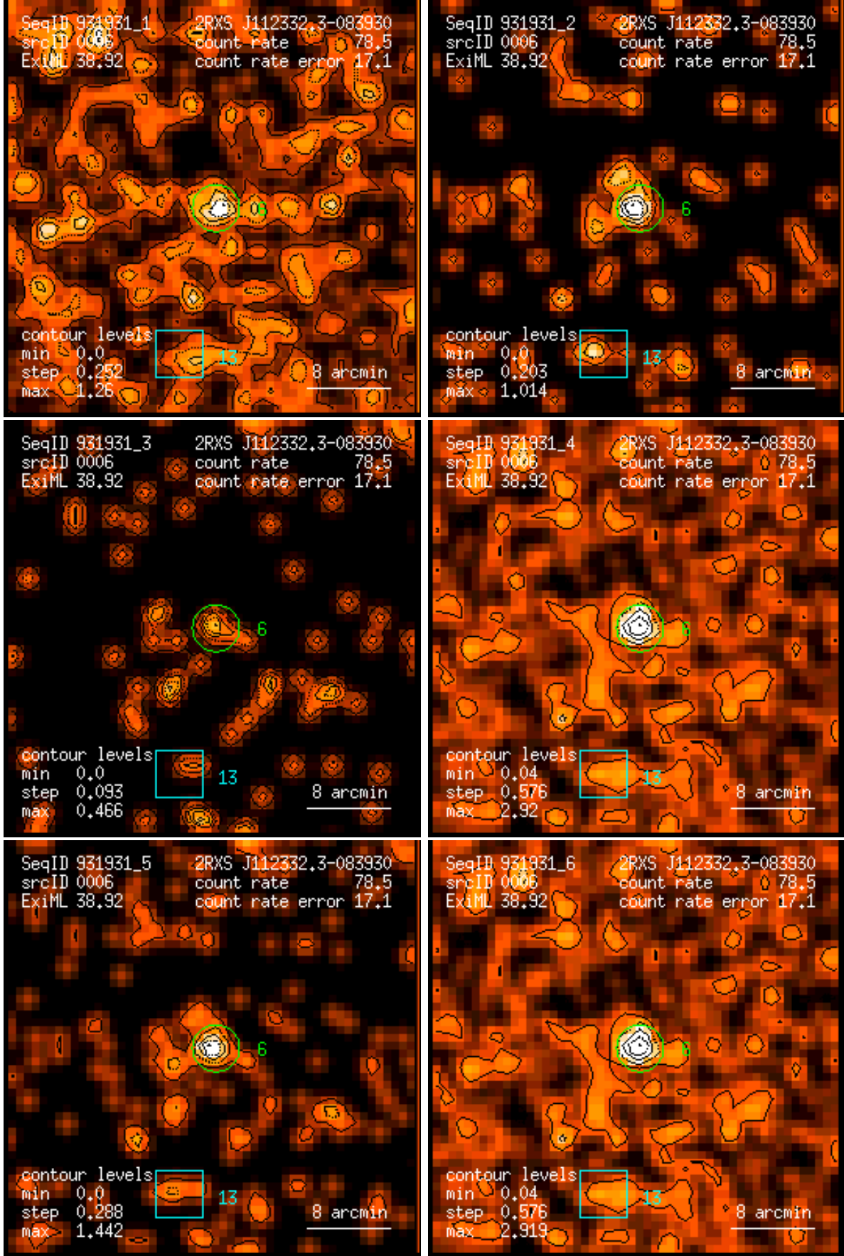
Figure 6: RASS 931931: detection 0006: band rate images, Gaussian filter: (1) PSPC channels 11 – 41, (2) 52 – 90, (3) 91 – 201, (4) 11 – 235, (5) 52 – 201, (6) 11 – 201. Broad band rates in counts/ks. Band rate contour levels in counts/ks/arcmin 2 .
