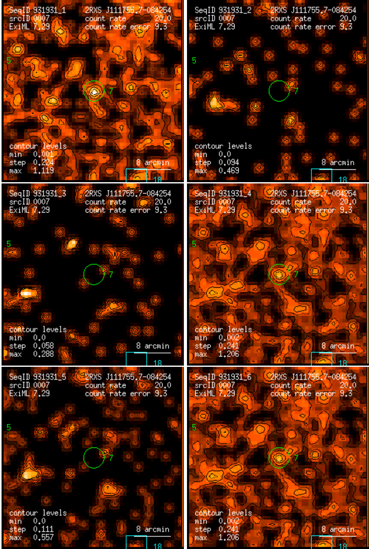
Figure 7: RASS 931931: detection 0007: band rate images, Gaussian filter: (1) PSPC channels 11 – 41, (2) 52 – 90, (3) 91 – 201, (4) 11 – 235, (5) 52 – 201, (6) 11 – 201. Broad band rates in counts/ks. Band rate contour levels in counts/ks/arcmin 2 .
