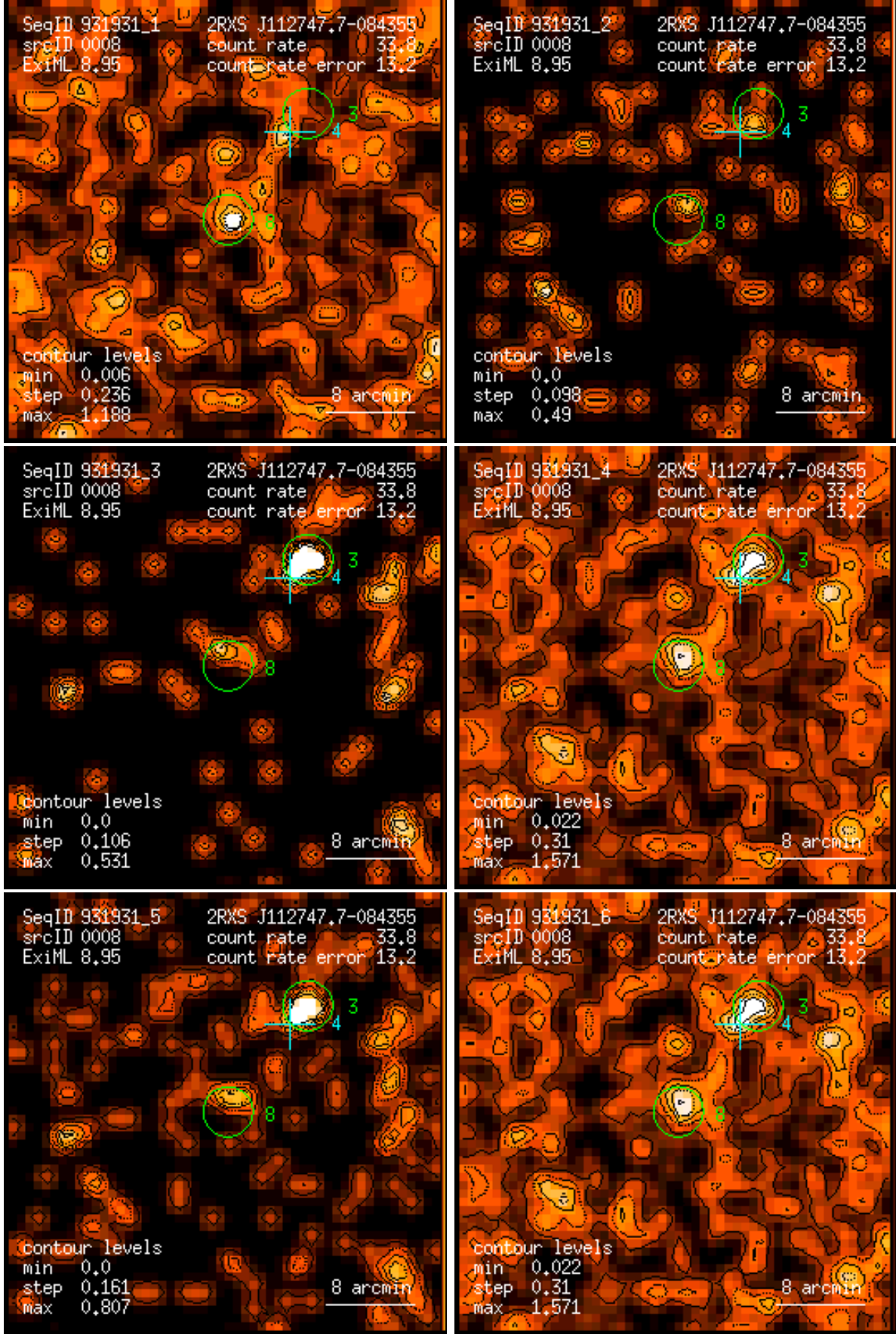
Figure 8: RASS 931931: detection 0008: band rate images, Gaussian filter: (1) PSPC channels 11 – 41, (2) 52 – 90, (3) 91 – 201, (4) 11 – 235, (5) 52 – 201, (6) 11 – 201. Broad band rates in counts/ks. Band rate contour levels in counts/ks/arcmin 2 .
