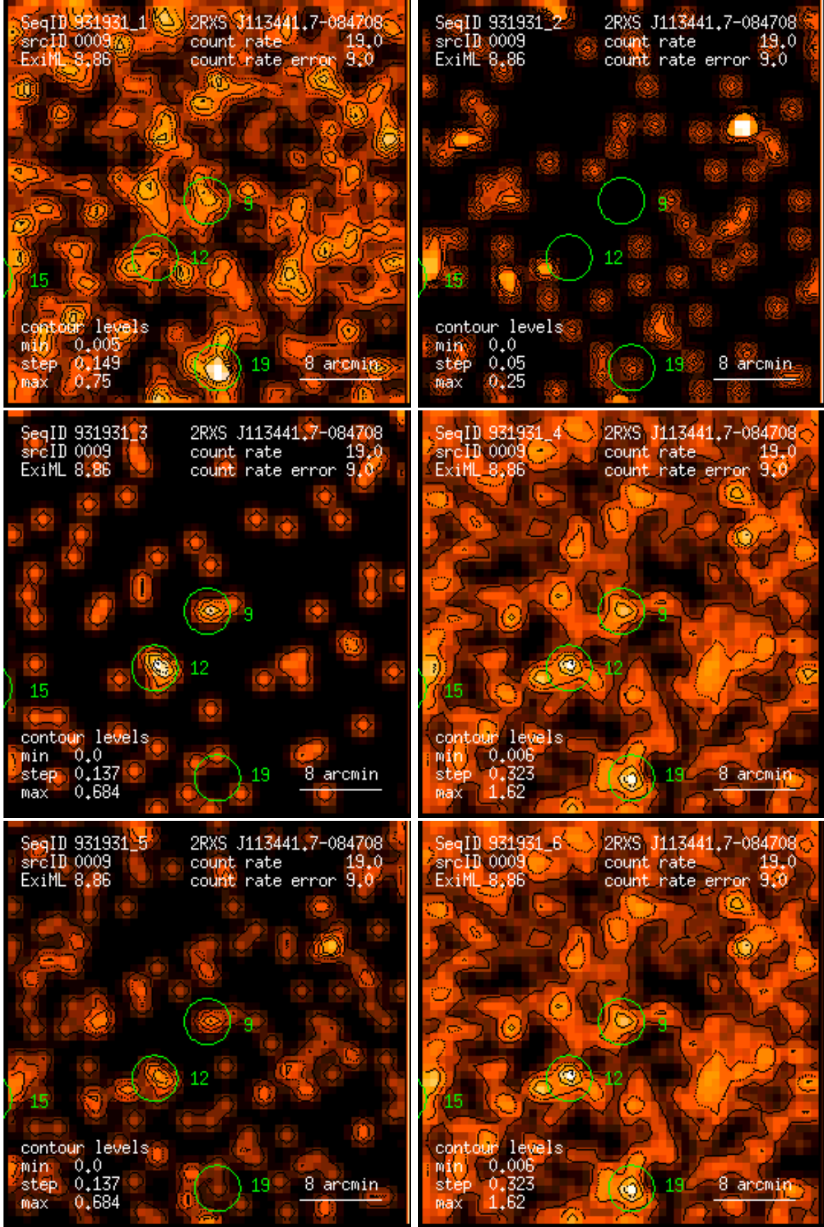
Figure 9: RASS 931931: detection 0009: band rate images, Gaussian filter: (1) PSPC channels 11 – 41, (2) 52 – 90, (3) 91 – 201, (4) 11 – 235, (5) 52 – 201, (6) 11 – 201. Broad band rates in counts/ks. Band rate contour levels in counts/ks/arcmin 2 .
