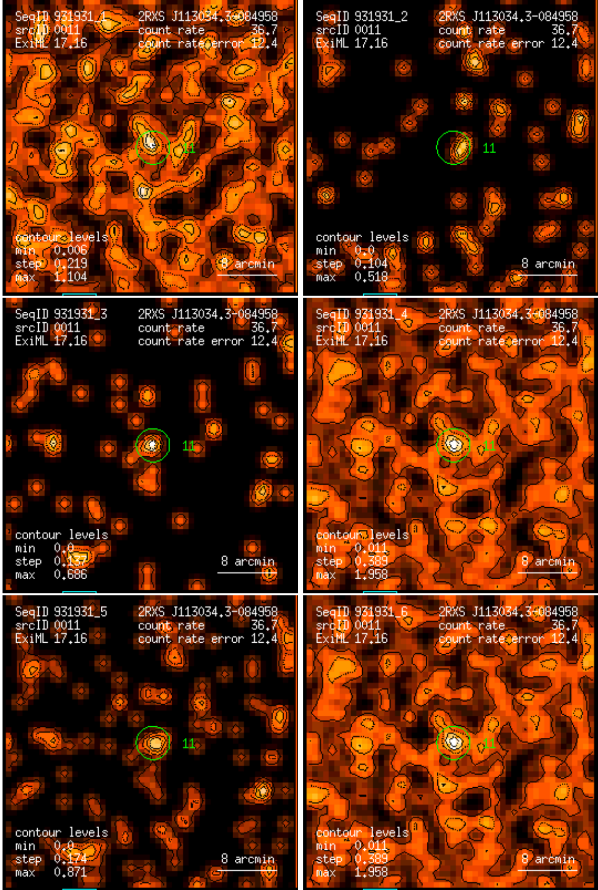
Figure 11: RASS 931931: detection 0011: band rate images, Gaussian filter: (1) PSPC channels 11 – 41, (2) 52 – 90, (3) 91 – 201, (4) 11 – 235, (5) 52 – 201, (6) 11 – 201. Broad band rates in counts/ks. Band rate contour levels in counts/ks/arcmin 2 .
