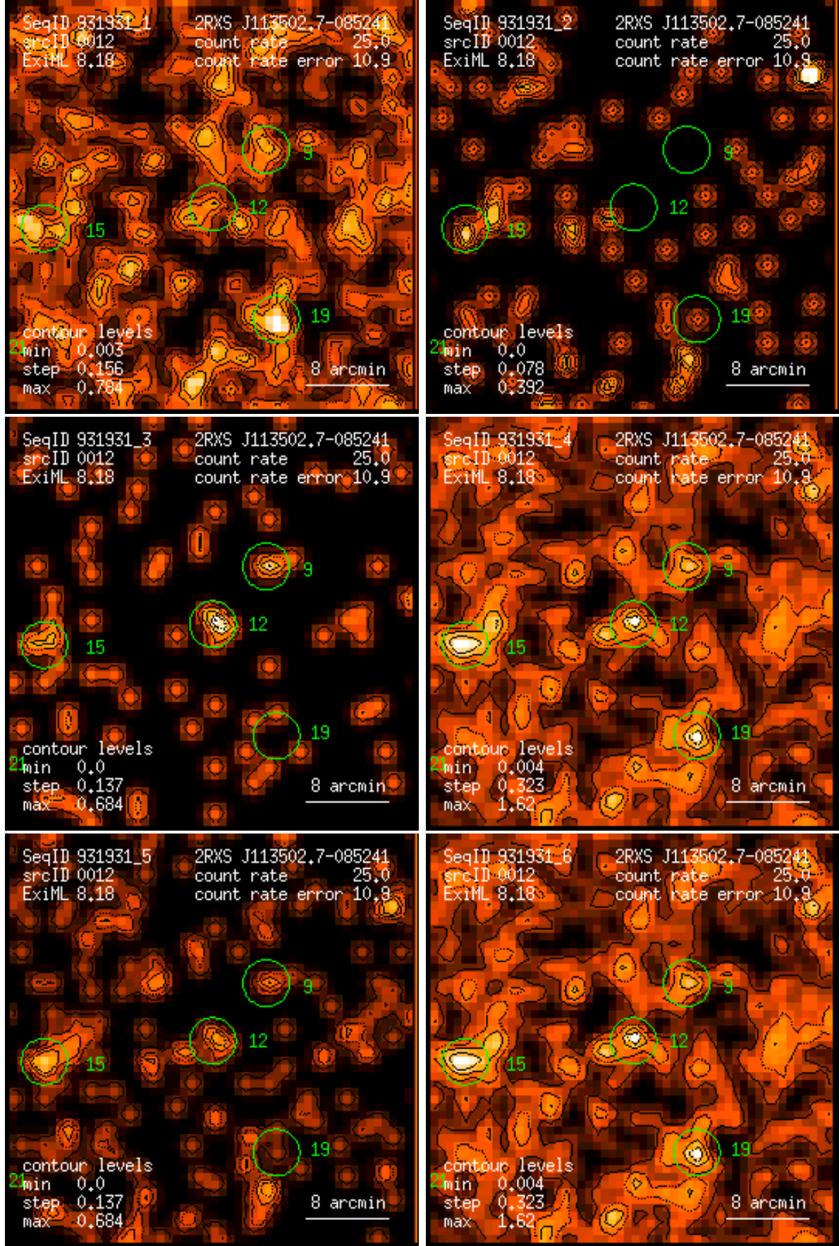
Figure 12: RASS 931931: detection 0012: band rate images, Gaussian filter: (1) PSPC channels 11 – 41, (2) 52 – 90, (3) 91 – 201, (4) 11 – 235, (5) 52 – 201, (6) 11 – 201. Broad band rates in counts/ks. Band rate contour levels in counts/ks/arcmin 2 .
