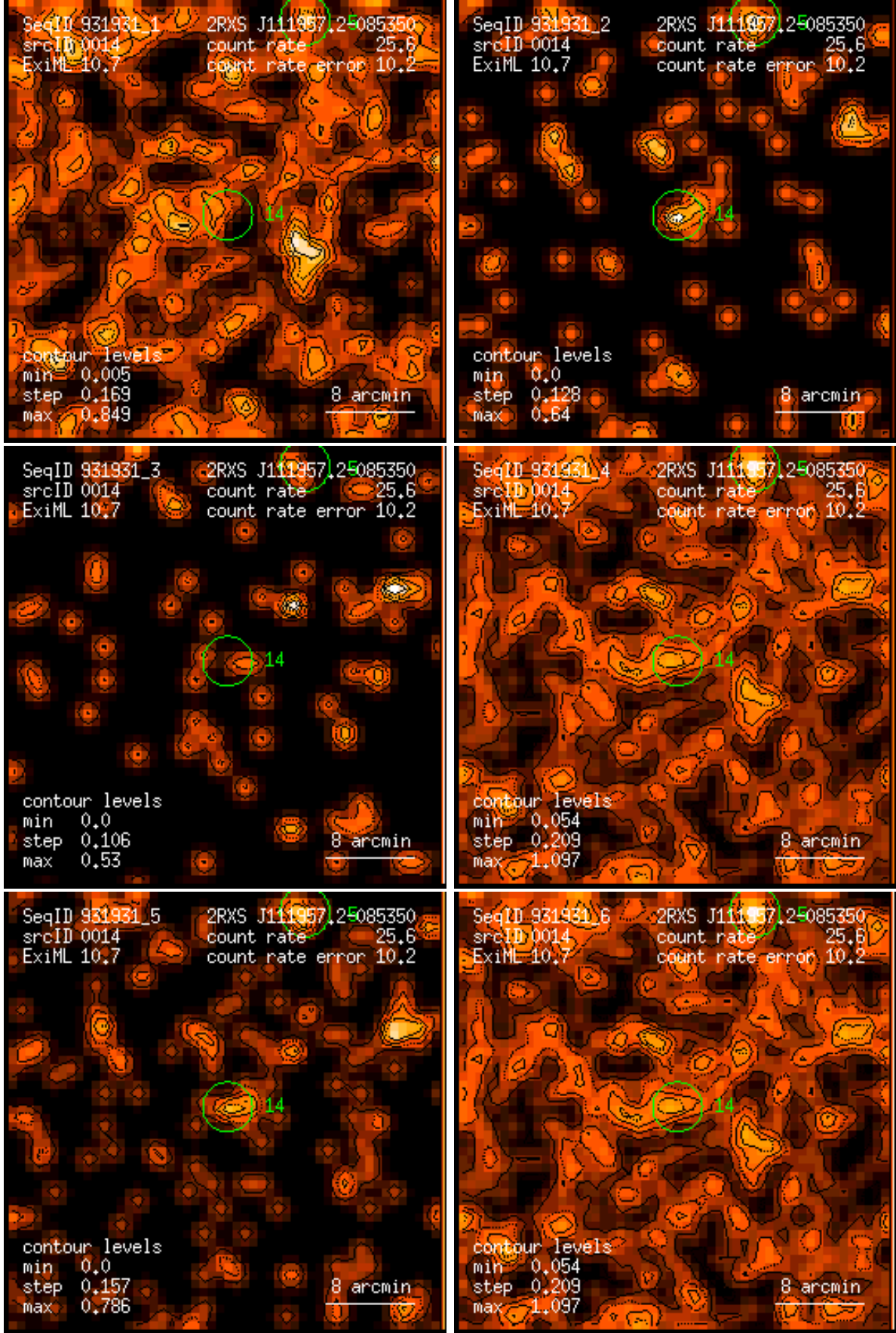
Figure 14: RASS 931931: detection 0014: band rate images, Gaussian filter: (1) PSPC channels 11 – 41, (2) 52 – 90, (3) 91 – 201, (4) 11 – 235, (5) 52 – 201, (6) 11 – 201. Broad band rates in counts/ks. Band rate contour levels in counts/ks/arcmin 2 .
