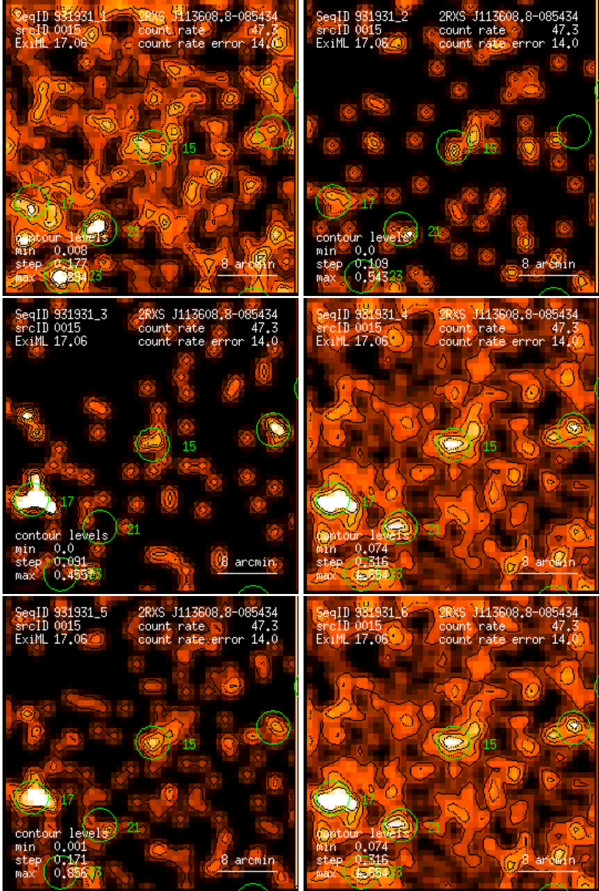
Figure 15: RASS 931931: detection 0015: band rate images, Gaussian filter: (1) PSPC channels 11 – 41, (2) 52 – 90, (3) 91 – 201, (4) 11 – 235, (5) 52 – 201, (6) 11 – 201. Broad band rates in counts/ks. Band rate contour levels in counts/ks/arcmin 2 .
