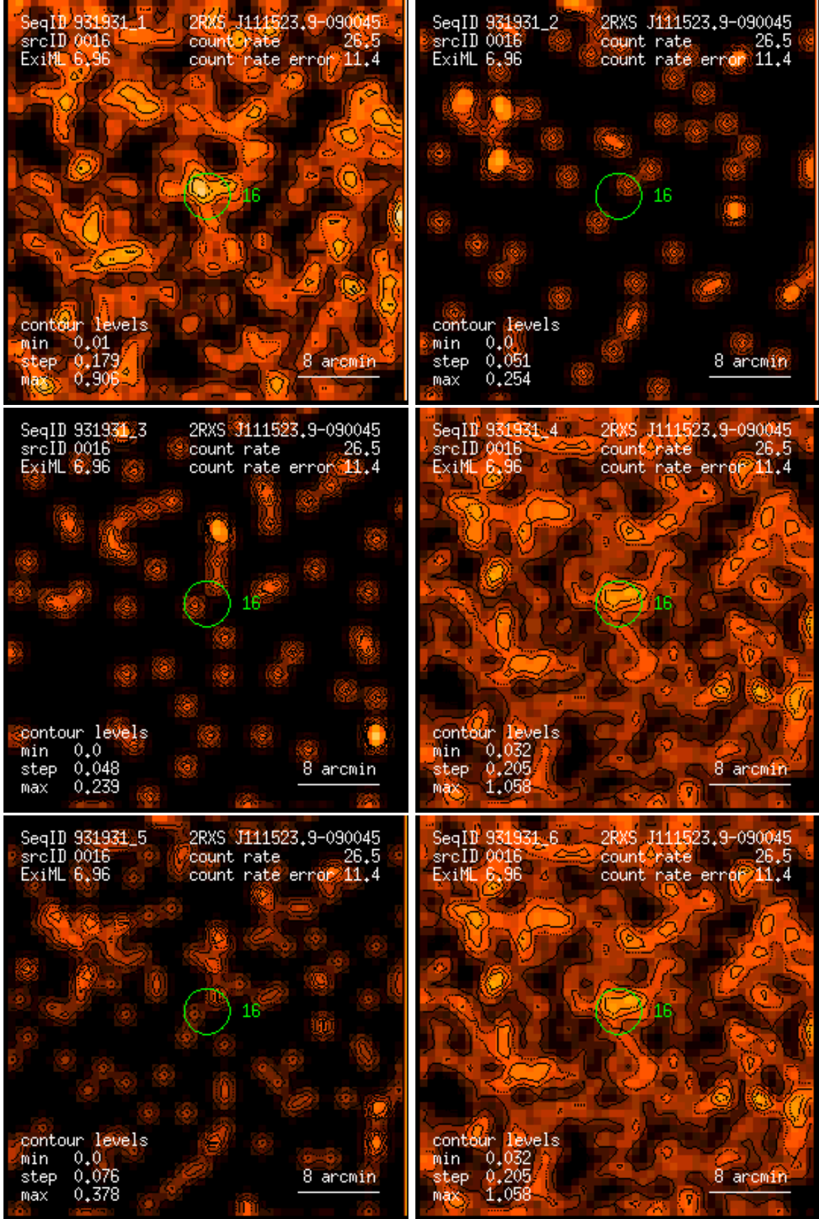
Figure 16: RASS 931931: detection 0016: band rate images, Gaussian filter: (1) PSPC channels 11 – 41, (2) 52 – 90, (3) 91 – 201, (4) 11 – 235, (5) 52 – 201, (6) 11 – 201. Broad band rates in counts/ks. Band rate contour levels in counts/ks/arcmin 2 .
