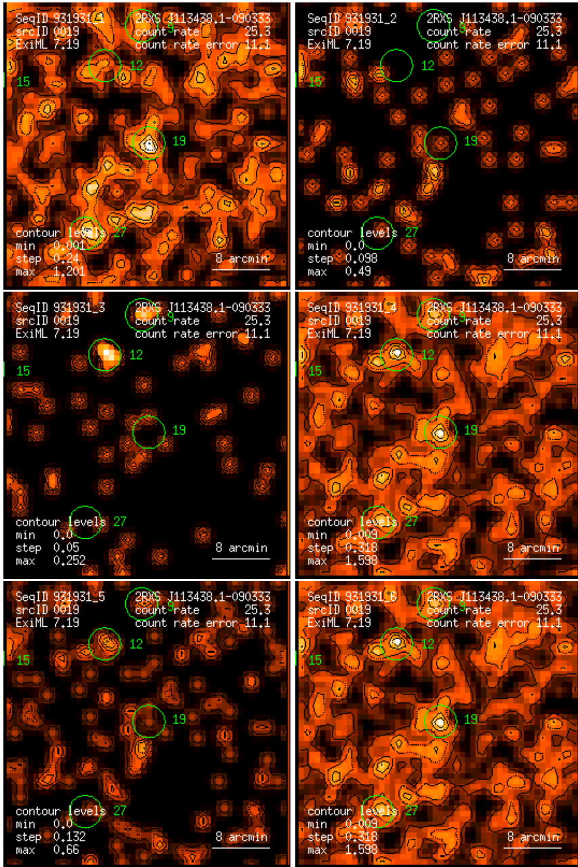
Figure 19: RASS 931931: detection 0019: band rate images, Gaussian filter: (1) PSPC channels 11 – 41, (2) 52 – 90, (3) 91 – 201, (4) 11 – 235, (5) 52 – 201, (6) 11 – 201. Broad band rates in counts/ks. Band rate contour levels in counts/ks/arcmin 2 .
