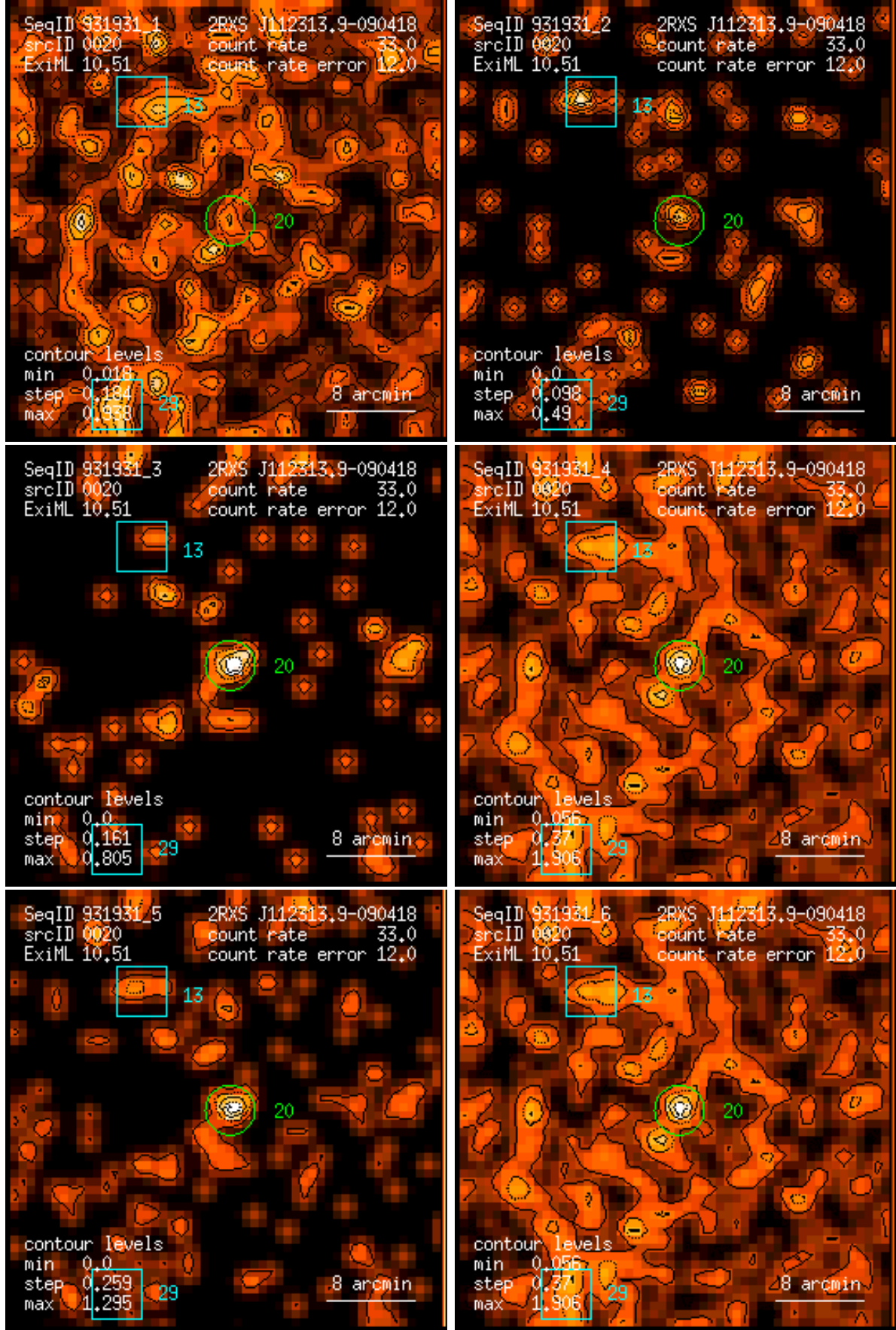
Figure 20: RASS 931931: detection 0020: band rate images, Gaussian filter: (1) PSPC channels 11 – 41, (2) 52 – 90, (3) 91 – 201, (4) 11 – 235, (5) 52 – 201, (6) 11 – 201. Broad band rates in counts/ks. Band rate contour levels in counts/ks/arcmin 2 .
