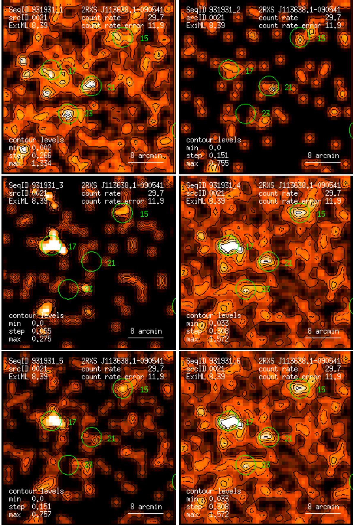
Figure 21: RASS 931931: detection 0021: band rate images, Gaussian filter: (1) PSPC channels 11 – 41, (2) 52 – 90, (3) 91 – 201, (4) 11 – 235, (5) 52 – 201, (6) 11 – 201. Broad band rates in counts/ks. Band rate contour levels in counts/ks/arcmin 2 .
