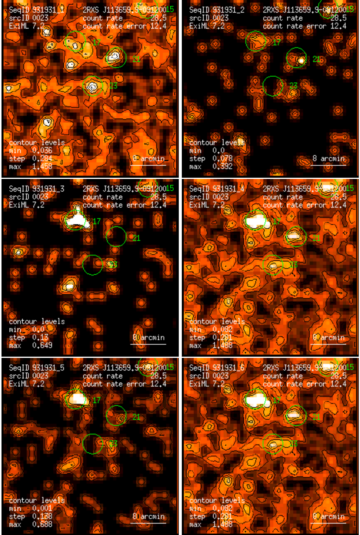
Figure 23: RASS 931931: detection 0023: band rate images, Gaussian filter: (1) PSPC channels 11 – 41, (2) 52 – 90, (3) 91 – 201, (4) 11 – 235, (5) 52 – 201, (6) 11 – 201. Broad band rates in counts/ks. Band rate contour levels in counts/ks/arcmin 2 .
