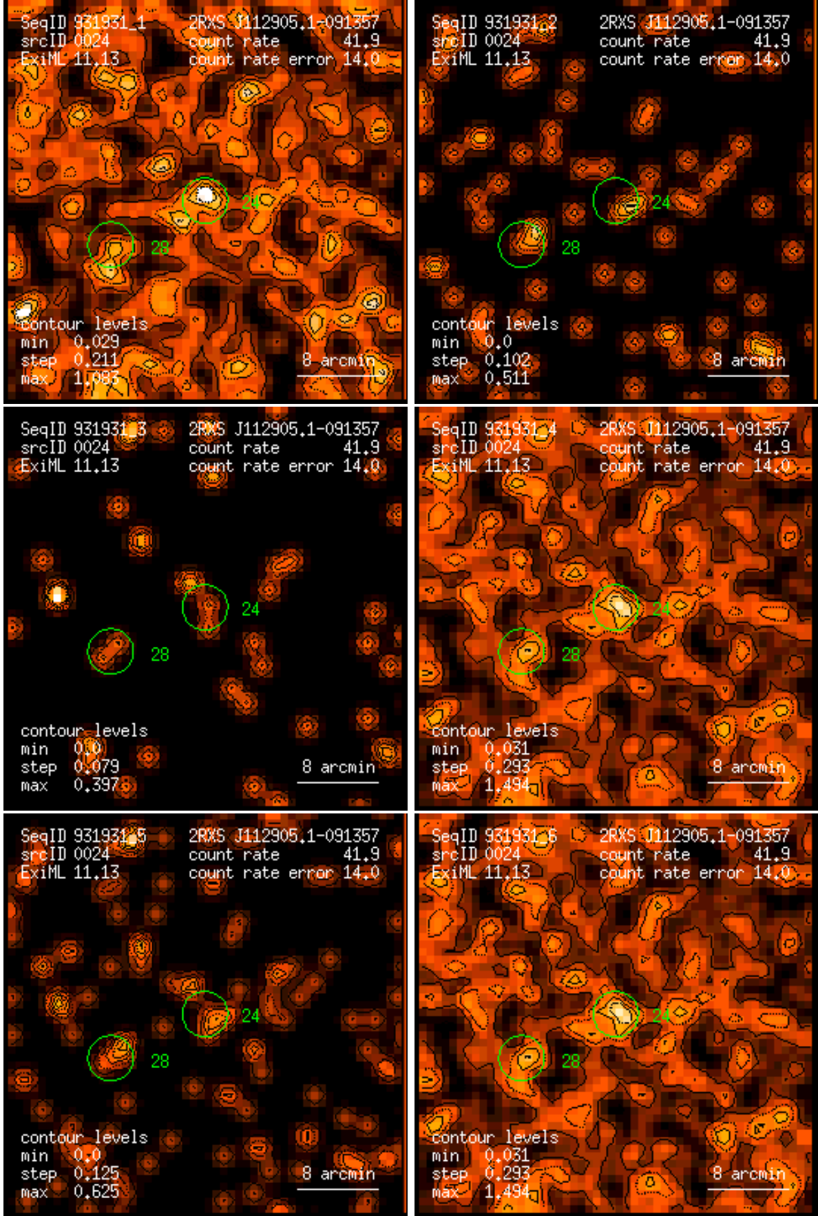
Figure 24: RASS 931931: detection 0024: band rate images, Gaussian filter: (1) PSPC channels 11 – 41, (2) 52 – 90, (3) 91 – 201, (4) 11 – 235, (5) 52 – 201, (6) 11 – 201. Broad band rates in counts/ks. Band rate contour levels in counts/ks/arcmin 2 .
