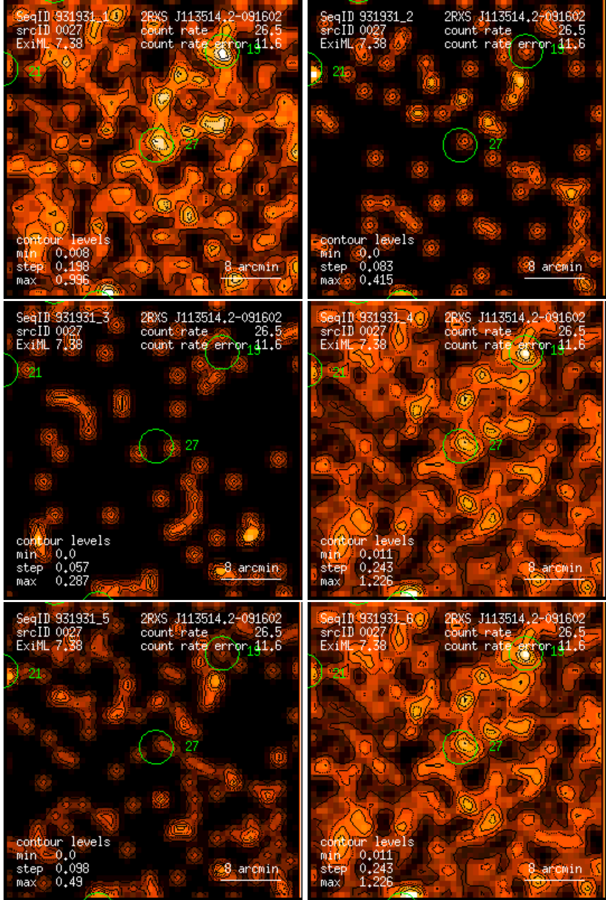
Figure 27: RASS 931931: detection 0027: band rate images, Gaussian filter: (1) PSPC channels 11 – 41, (2) 52 – 90, (3) 91 – 201, (4) 11 – 235, (5) 52 – 201, (6) 11 – 201. Broad band rates in counts/ks. Band rate contour levels in counts/ks/arcmin 2 .
