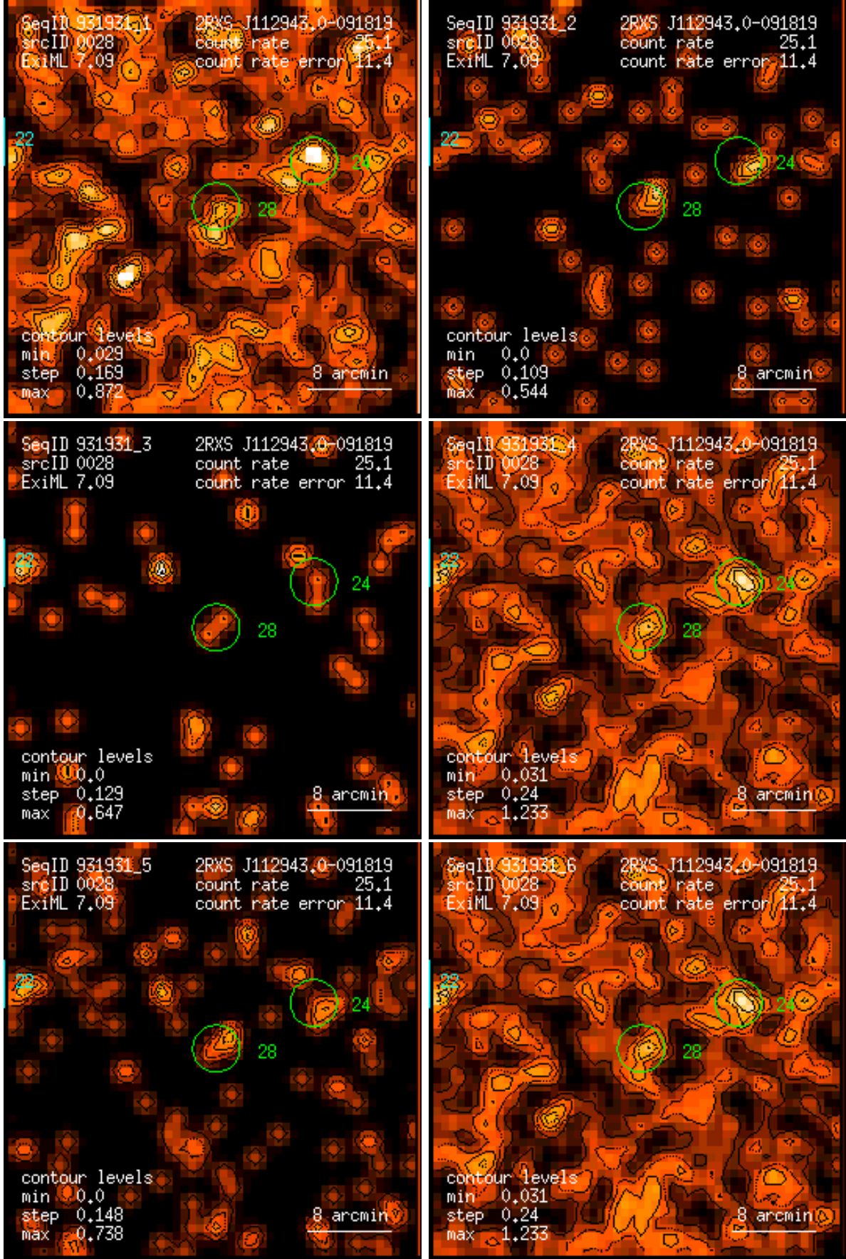
Figure 28: RASS 931931: detection 0028: band rate images, Gaussian filter: (1) PSPC channels 11 – 41, (2) 52 – 90, (3) 91 – 201, (4) 11 – 235, (5) 52 – 201, (6) 11 – 201. Broad band rates in counts/ks. Band rate contour levels in counts/ks/arcmin 2 .
