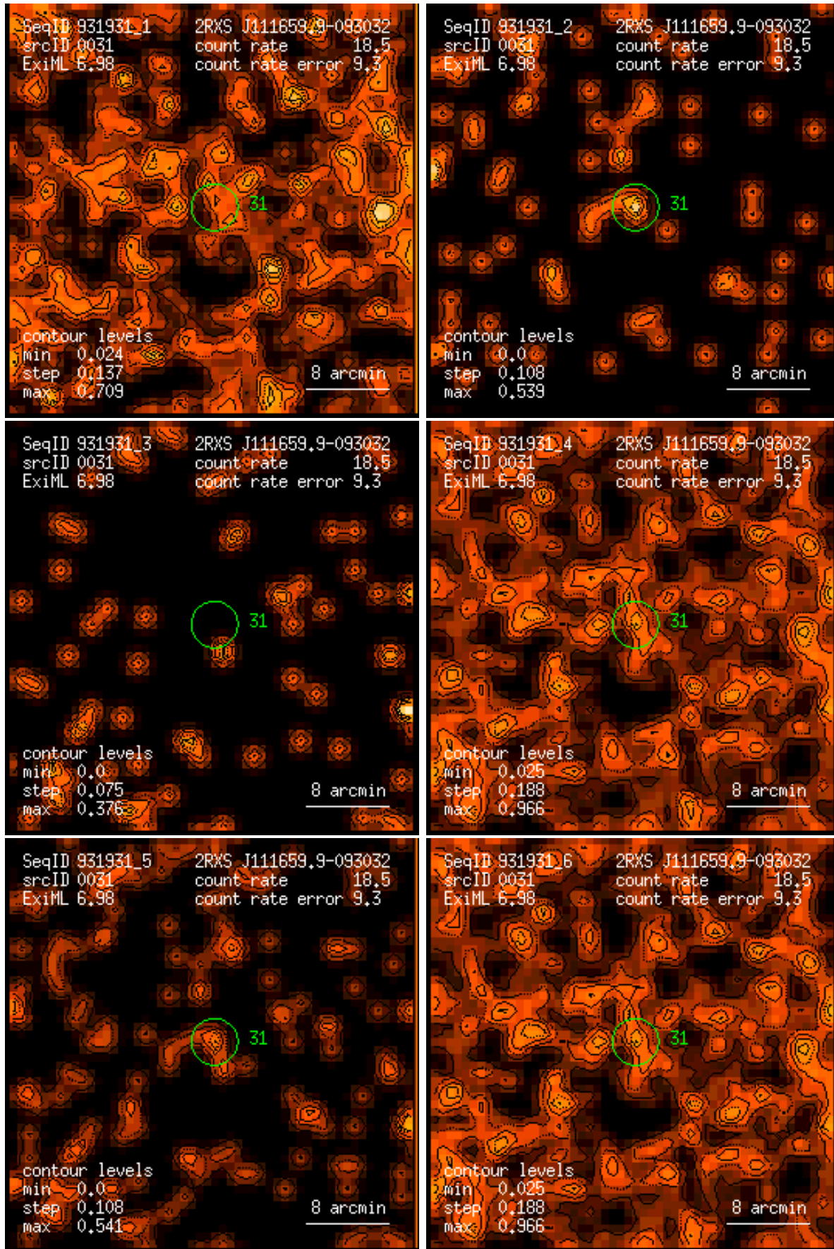
Figure 31: RASS 931931: detection 0031: band rate images, Gaussian filter: (1) PSPC channels 11 – 41, (2) 52 – 90, (3) 91 – 201, (4) 11 – 235, (5) 52 – 201, (6) 11 – 201. Broad band rates in counts/ks. Band rate contour levels in counts/ks/arcmin 2 .
