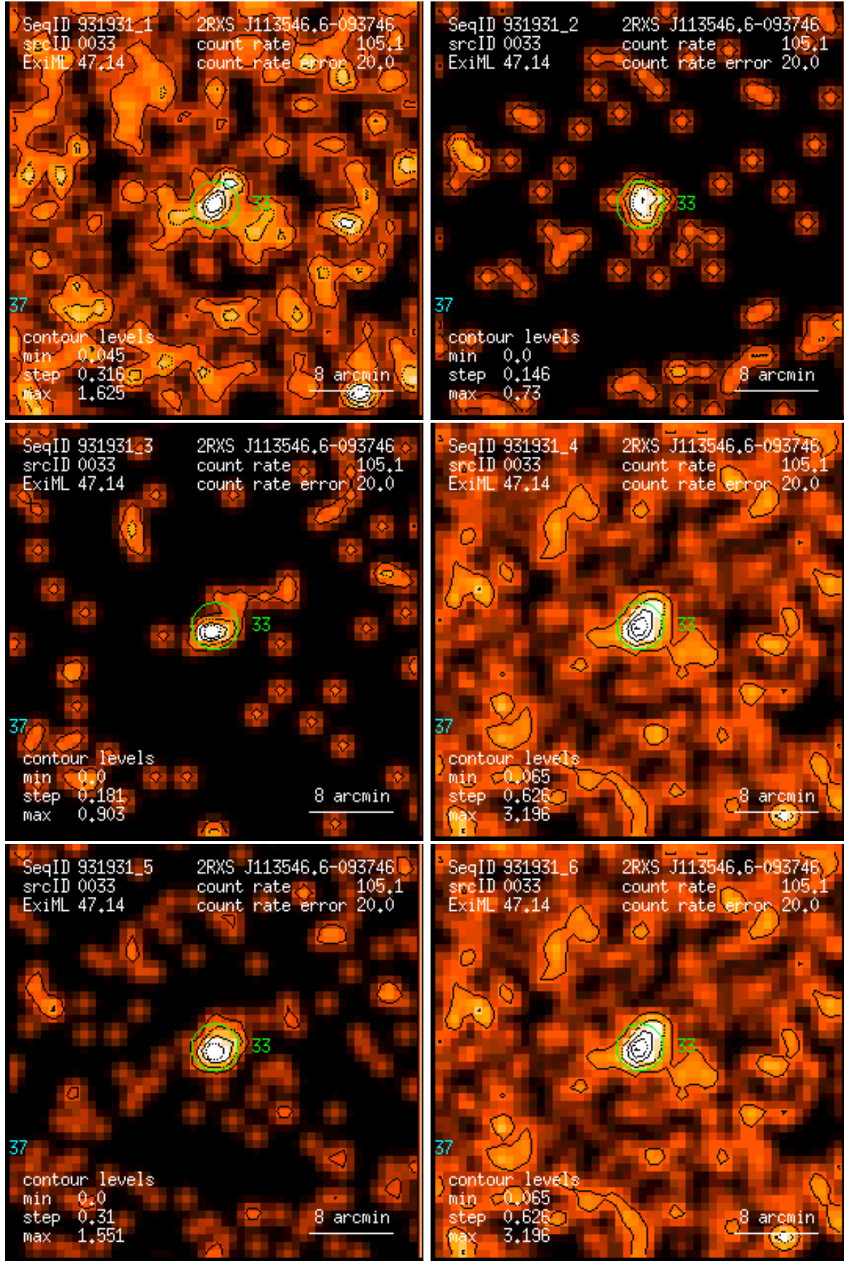
Figure 33: RASS 931931: detection 0033: band rate images, Gaussian filter: (1) PSPC channels 11 – 41, (2) 52 – 90, (3) 91 – 201, (4) 11 – 235, (5) 52 – 201, (6) 11 – 201. Broad band rates in counts/ks. Band rate contour levels in counts/ks/arcmin 2 .
