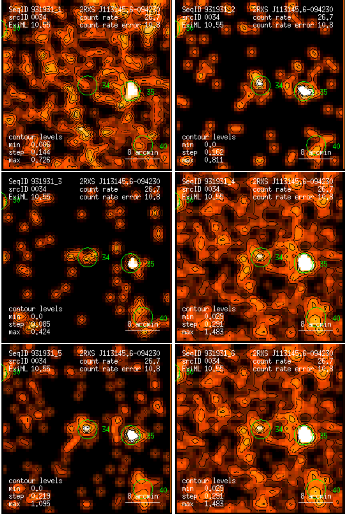
Figure 34: RASS 931931: detection 0034: band rate images, Gaussian filter: (1) PSPC channels 11 – 41, (2) 52 – 90, (3) 91 – 201, (4) 11 – 235, (5) 52 – 201, (6) 11 – 201. Broad band rates in counts/ks. Band rate contour levels in counts/ks/arcmin 2 .
