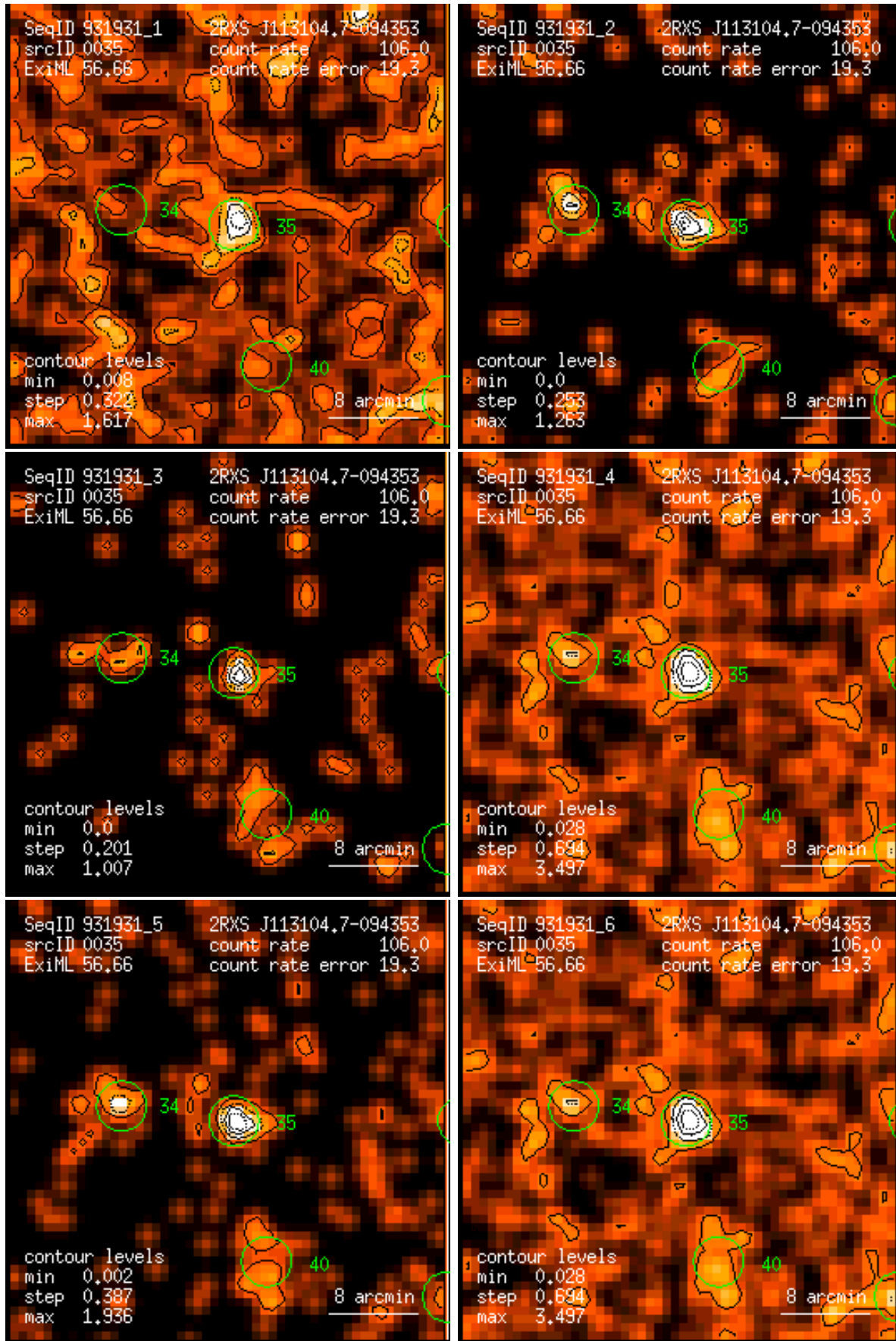
Figure 35: RASS 931931: detection 0035: band rate images, Gaussian filter: (1) PSPC channels 11 – 41, (2) 52 – 90, (3) 91 – 201, (4) 11 – 235, (5) 52 – 201, (6) 11 – 201. Broad band rates in counts/ks. Band rate contour levels in counts/ks/arcmin 2 .
