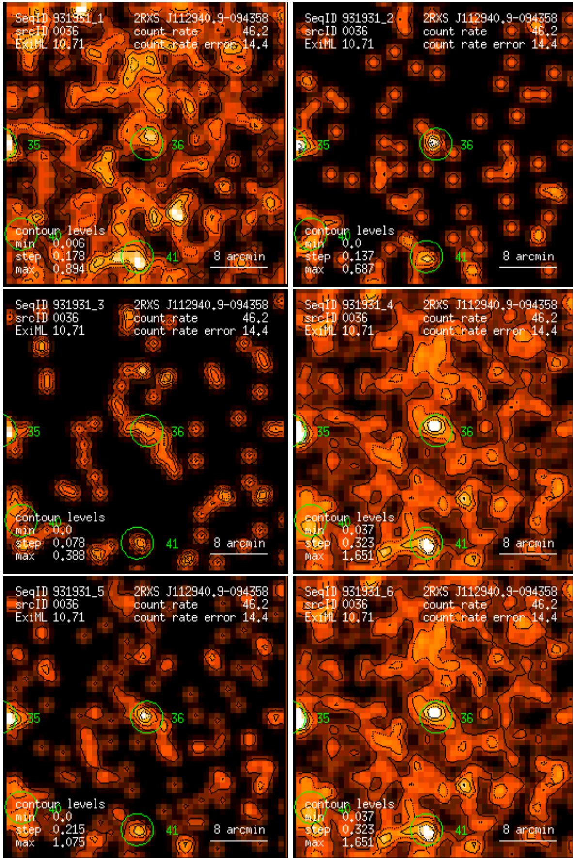
Figure 36: RASS 931931: detection 0036: band rate images, Gaussian filter: (1) PSPC channels 11 – 41, (2) 52 – 90, (3) 91 – 201, (4) 11 – 235, (5) 52 – 201, (6) 11 – 201. Broad band rates in counts/ks. Band rate contour levels in counts/ks/arcmin 2 .
