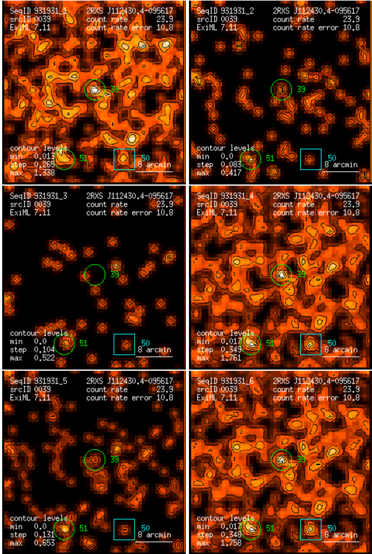
Figure 39: RASS 931931: detection 0039: band rate images, Gaussian filter: (1) PSPC channels 11 – 41, (2) 52 – 90, (3) 91 – 201, (4) 11 – 235, (5) 52 – 201, (6) 11 – 201. Broad band rates in counts/ks. Band rate contour levels in counts/ks/arcmin 2 .
