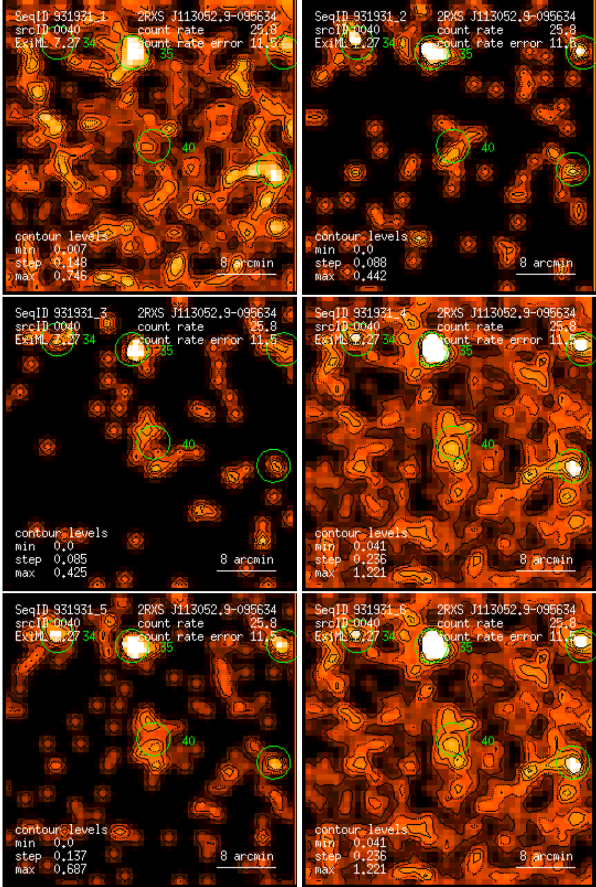
Figure 40: RASS 931931: detection 0040: band rate images, Gaussian filter: (1) PSPC channels 11 – 41, (2) 52 – 90, (3) 91 – 201, (4) 11 – 235, (5) 52 – 201, (6) 11 – 201. Broad band rates in counts/ks. Band rate contour levels in counts/ks/arcmin 2 .
