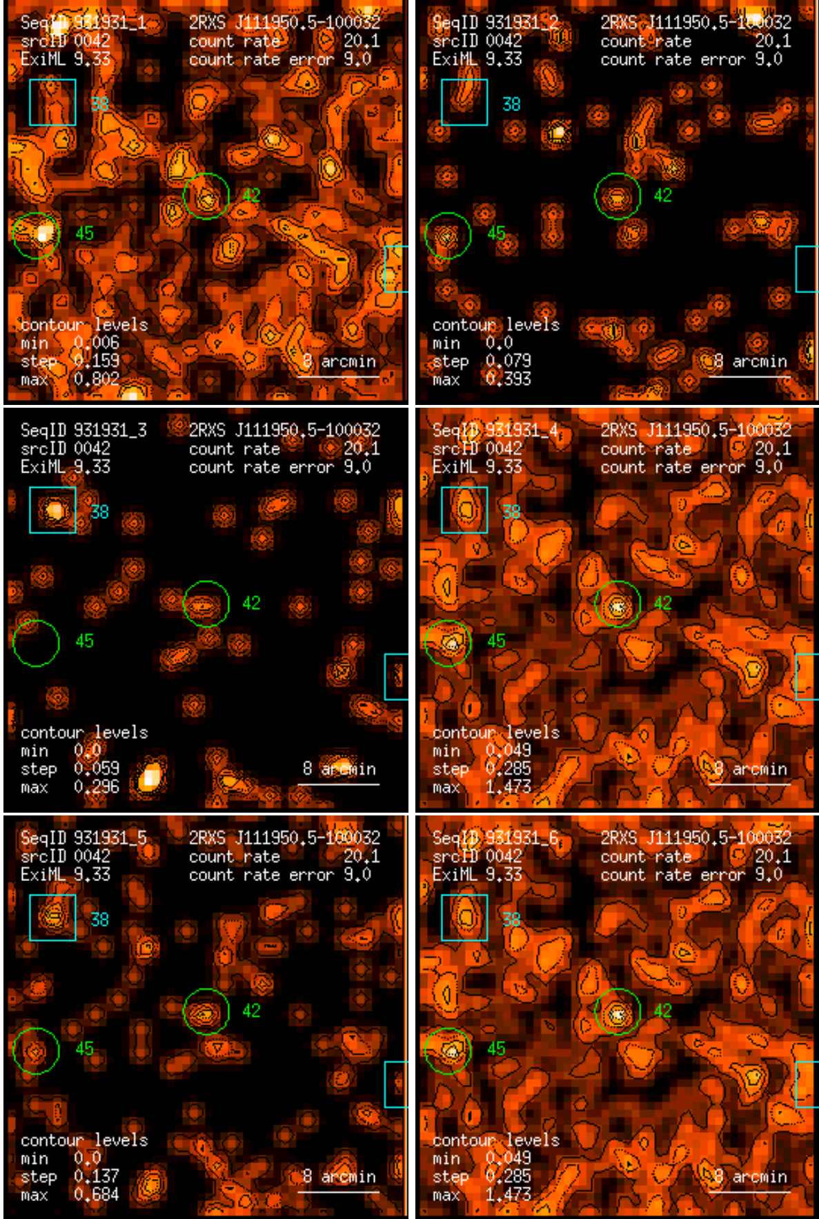
Figure 42: RASS 931931: detection 0042: band rate images, Gaussian filter: (1) PSPC channels 11 – 41, (2) 52 – 90, (3) 91 – 201, (4) 11 – 235, (5) 52 – 201, (6) 11 – 201. Broad band rates in counts/ks. Band rate contour levels in counts/ks/arcmin 2 .
