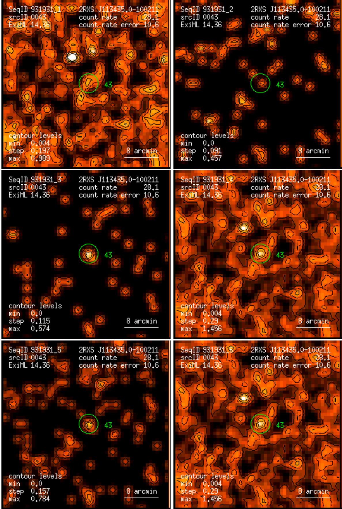
Figure 43: RASS 931931: detection 0043: band rate images, Gaussian filter: (1) PSPC channels 11 – 41, (2) 52 – 90, (3) 91 – 201, (4) 11 – 235, (5) 52 – 201, (6) 11 – 201. Broad band rates in counts/ks. Band rate contour levels in counts/ks/arcmin 2 .
