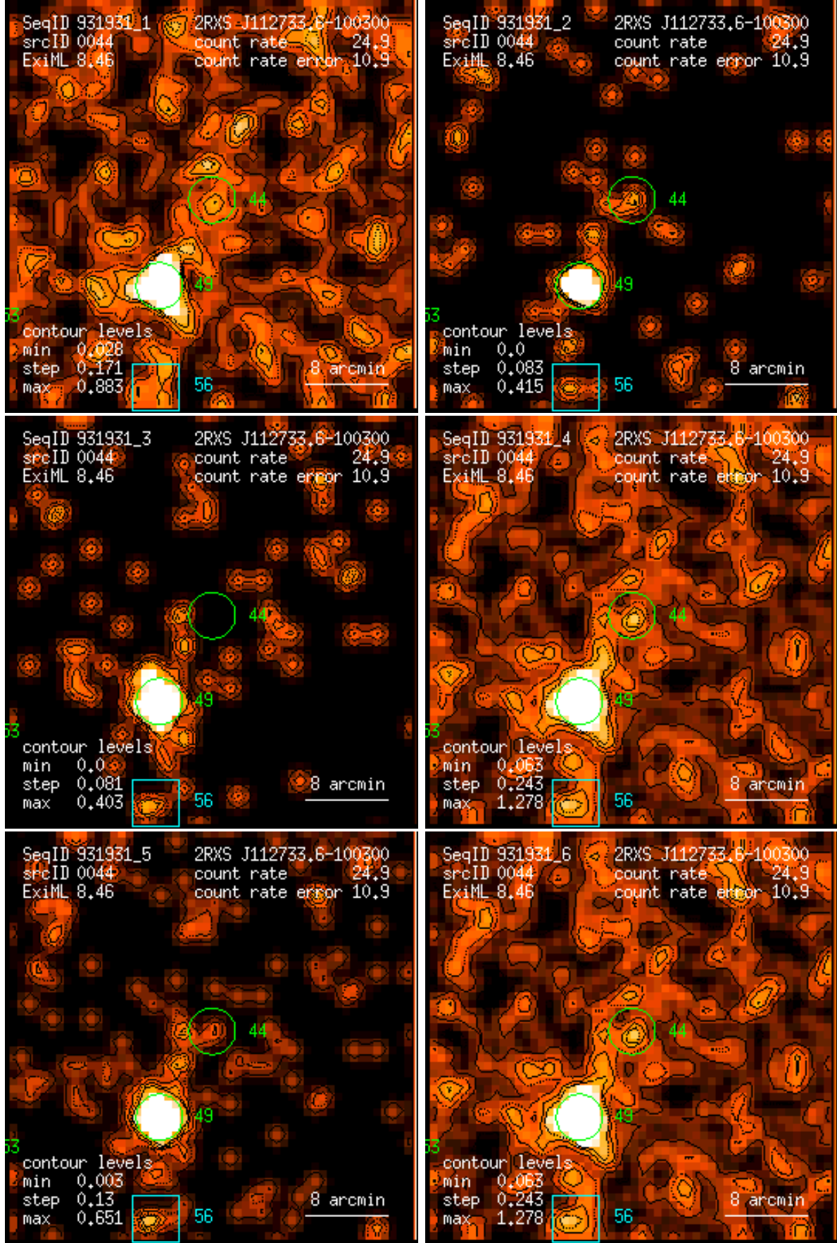
Figure 44: RASS 931931: detection 0044: band rate images, Gaussian filter: (1) PSPC channels 11 – 41, (2) 52 – 90, (3) 91 – 201, (4) 11 – 235, (5) 52 – 201, (6) 11 – 201. Broad band rates in counts/ks. Band rate contour levels in counts/ks/arcmin 2 .
