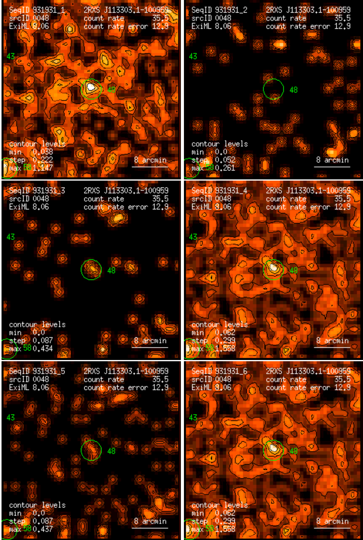
Figure 48: RASS 931931: detection 0048: band rate images, Gaussian filter: (1) PSPC channels 11 – 41, (2) 52 – 90, (3) 91 – 201, (4) 11 – 235, (5) 52 – 201, (6) 11 – 201. Broad band rates in counts/ks. Band rate contour levels in counts/ks/arcmin 2 .
