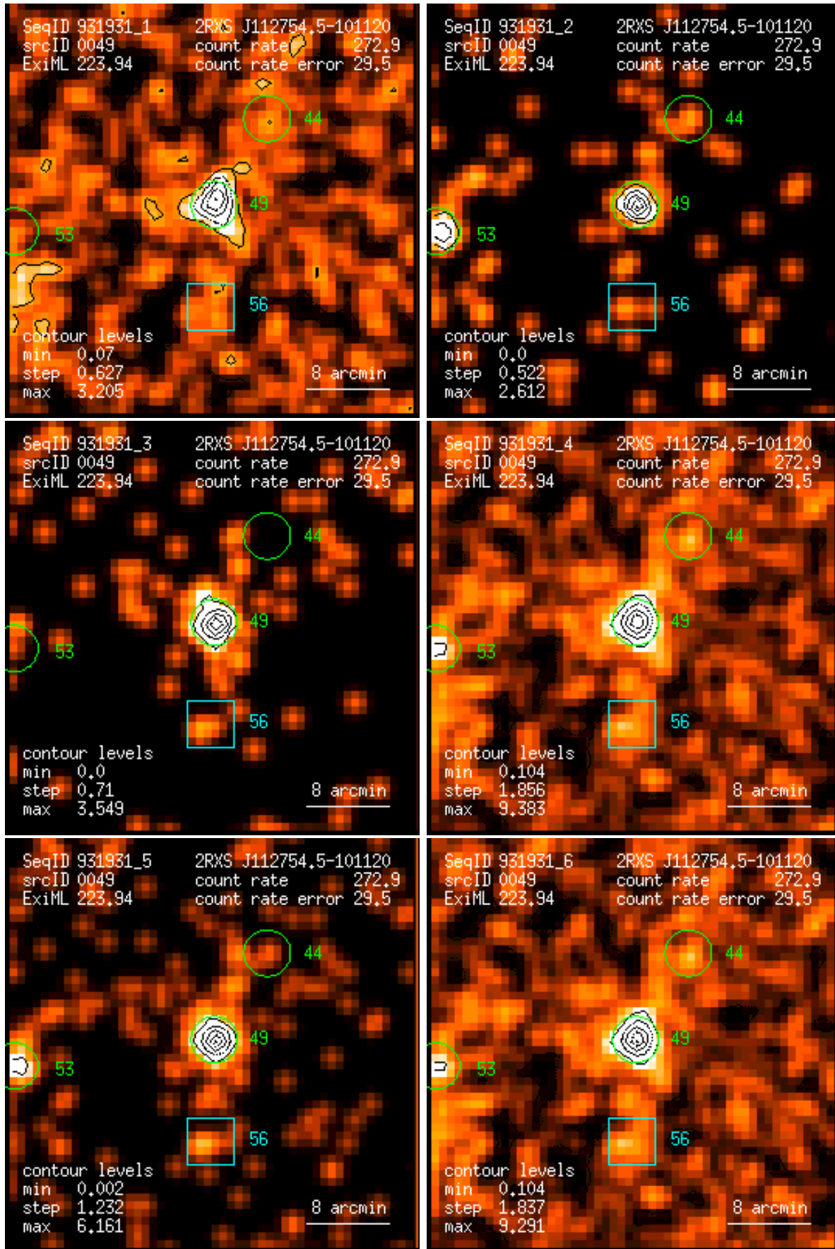
Figure 49: RASS 931931: detection 0049: band rate images, Gaussian filter: (1) PSPC channels 11 – 41, (2) 52 – 90, (3) 91 – 201, (4) 11 – 235, (5) 52 – 201, (6) 11 – 201. Broad band rates in counts/ks. Band rate contour levels in counts/ks/arcmin 2 .
