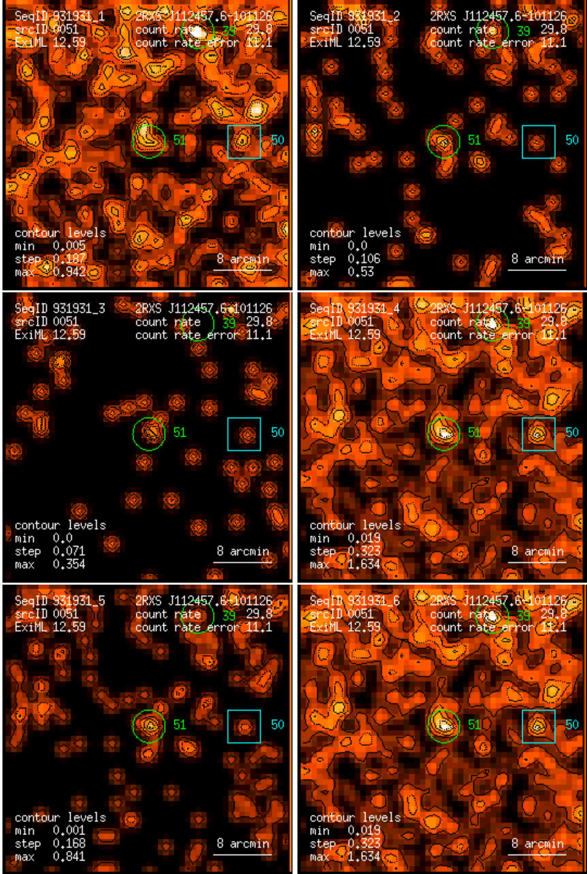
Figure 51: RASS 931931: detection 0051: band rate images, Gaussian filter: (1) PSPC channels 11 – 41, (2) 52 – 90, (3) 91 – 201, (4) 11 – 235, (5) 52 – 201, (6) 11 – 201. Broad band rates in counts/ks. Band rate contour levels in counts/ks/arcmin 2 .
