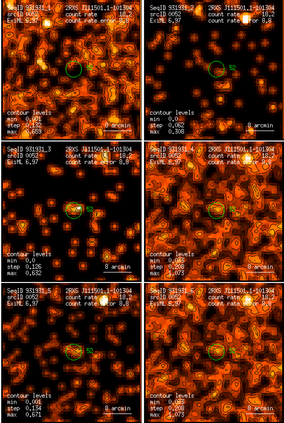
Figure 52: RASS 931931: detection 0052: band rate images, Gaussian filter: (1) PSPC channels 11 – 41, (2) 52 – 90, (3) 91 – 201, (4) 11 – 235, (5) 52 – 201, (6) 11 – 201. Broad band rates in counts/ks. Band rate contour levels in counts/ks/arcmin 2 .
