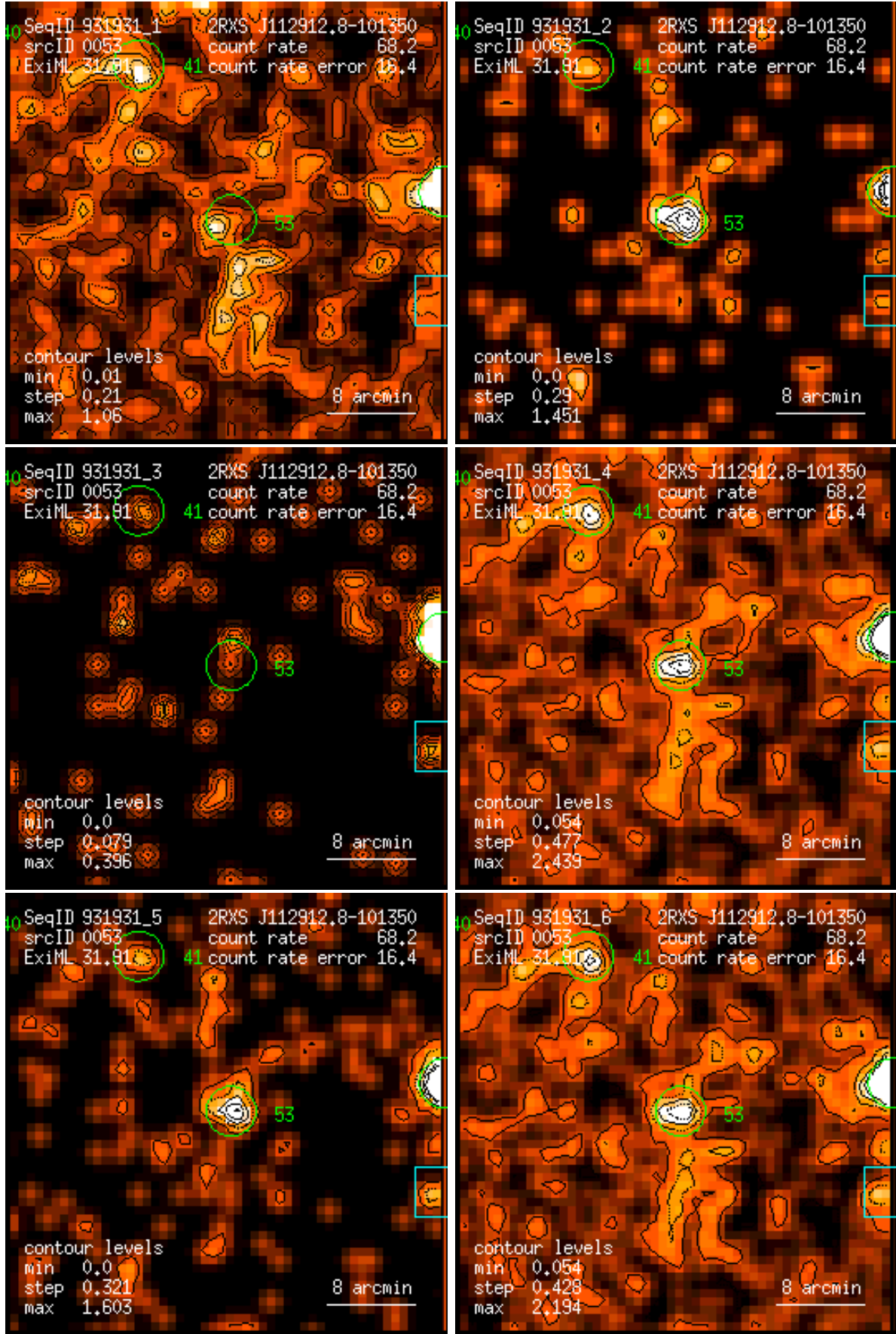
Figure 53: RASS 931931: detection 0053: band rate images, Gaussian filter: (1) PSPC channels 11 – 41, (2) 52 – 90, (3) 91 – 201, (4) 11 – 235, (5) 52 – 201, (6) 11 – 201. Broad band rates in counts/ks. Band rate contour levels in counts/ks/arcmin 2 .
