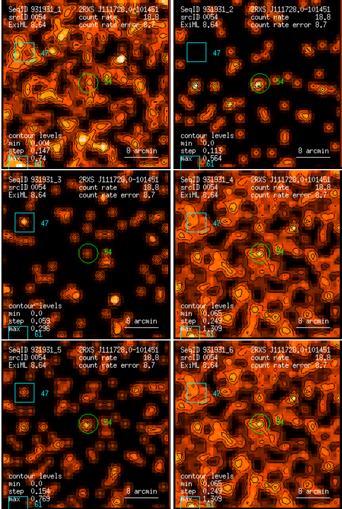
Figure 54: RASS 931931: detection 0054: band rate images, Gaussian filter: (1) PSPC channels 11 – 41, (2) 52 – 90, (3) 91 – 201, (4) 11 – 235, (5) 52 – 201, (6) 11 – 201. Broad band rates in counts/ks. Band rate contour levels in counts/ks/arcmin 2 .
