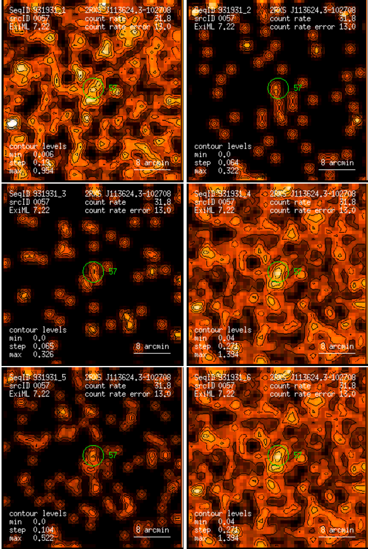
Figure 57: RASS 931931: detection 0057: band rate images, Gaussian filter: (1) PSPC channels 11 – 41, (2) 52 – 90, (3) 91 – 201, (4) 11 – 235, (5) 52 – 201, (6) 11 – 201. Broad band rates in counts/ks. Band rate contour levels in counts/ks/arcmin 2 .
