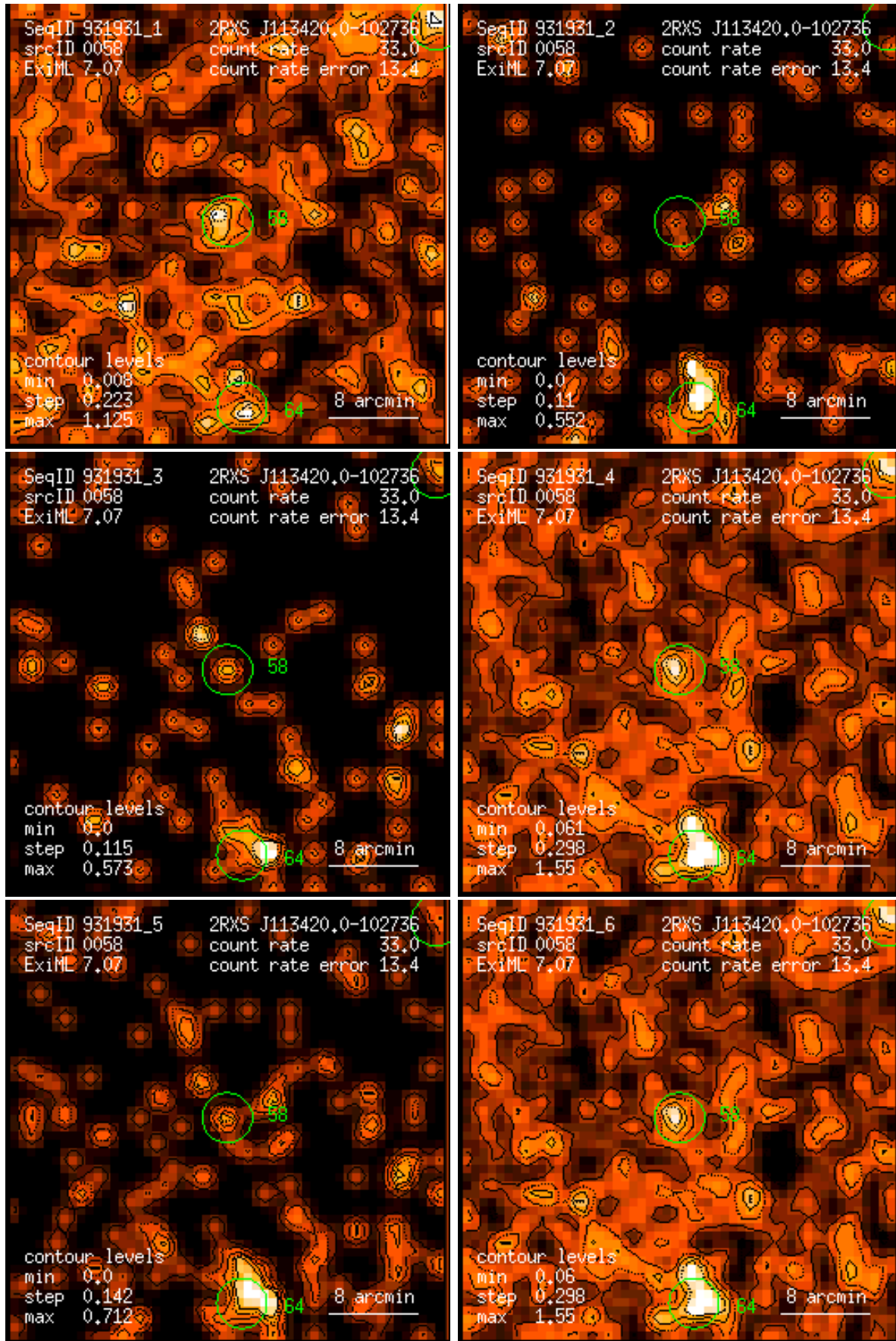
Figure 58: RASS 931931: detection 0058: band rate images, Gaussian filter: (1) PSPC channels 11 – 41, (2) 52 – 90, (3) 91 – 201, (4) 11 – 235, (5) 52 – 201, (6) 11 – 201. Broad band rates in counts/ks. Band rate contour levels in counts/ks/arcmin 2 .
