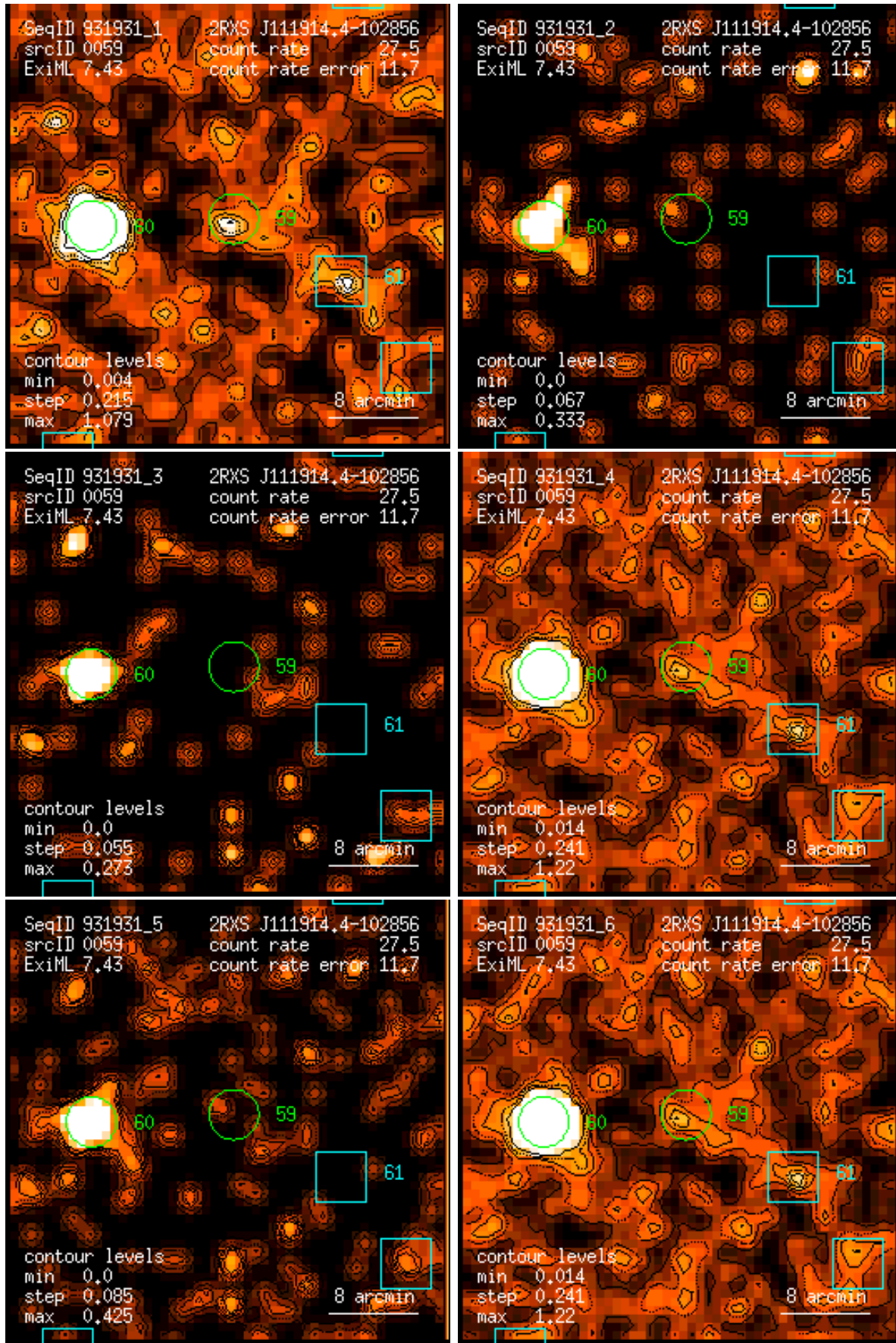
Figure 59: RASS 931931: detection 0059: band rate images, Gaussian filter: (1) PSPC channels 11 – 41, (2) 52 – 90, (3) 91 – 201, (4) 11 – 235, (5) 52 – 201, (6) 11 – 201. Broad band rates in counts/ks. Band rate contour levels in counts/ks/arcmin 2 .
