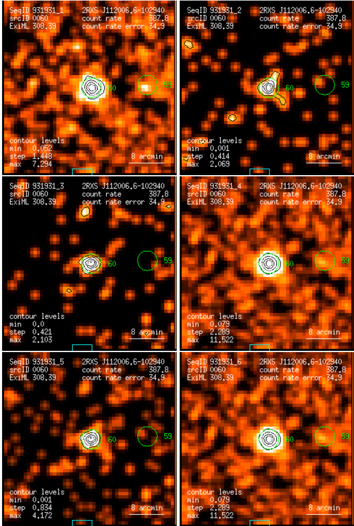
Figure 60: RASS 931931: detection 0060: band rate images, Gaussian filter: (1) PSPC channels 11 – 41, (2) 52 – 90, (3) 91 – 201, (4) 11 – 235, (5) 52 – 201, (6) 11 – 201. Broad band rates in counts/ks. Band rate contour levels in counts/ks/arcmin 2 .
