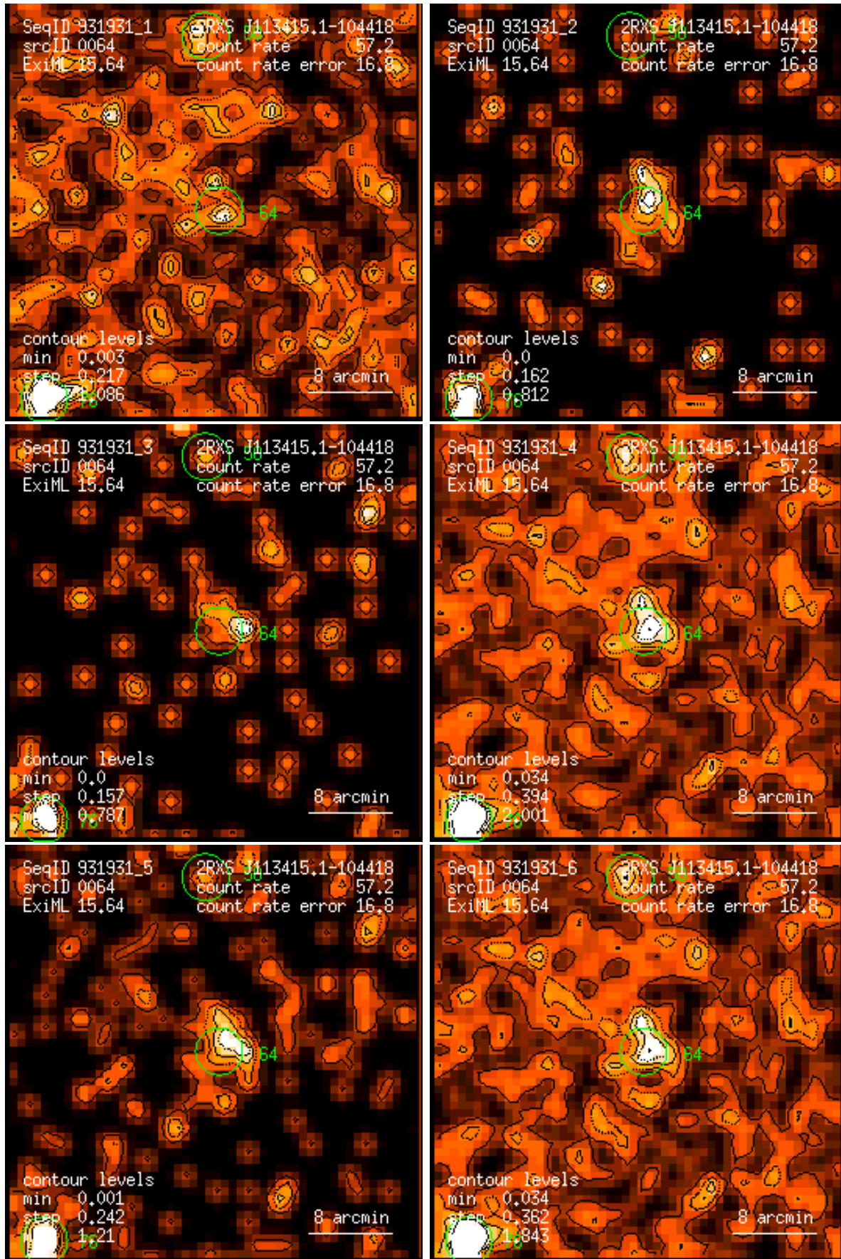
Figure 64: RASS 931931: detection 0064: band rate images, Gaussian filter: (1) PSPC channels 11 – 41, (2) 52 – 90, (3) 91 – 201, (4) 11 – 235, (5) 52 – 201, (6) 11 – 201. Broad band rates in counts/ks. Band rate contour levels in counts/ks/arcmin 2 .
